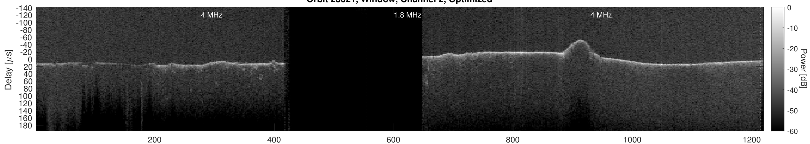
Orbit 23021, Cluttergram
