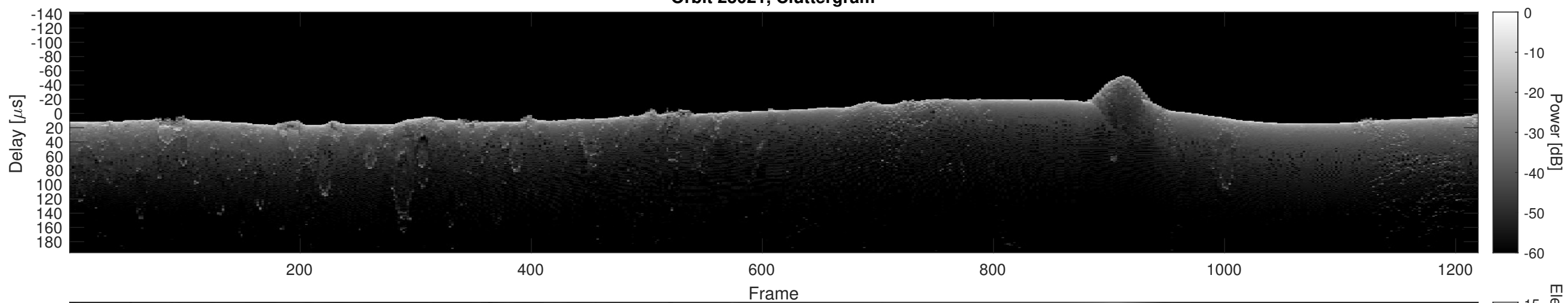
Orbit 23021, Cluttergram
