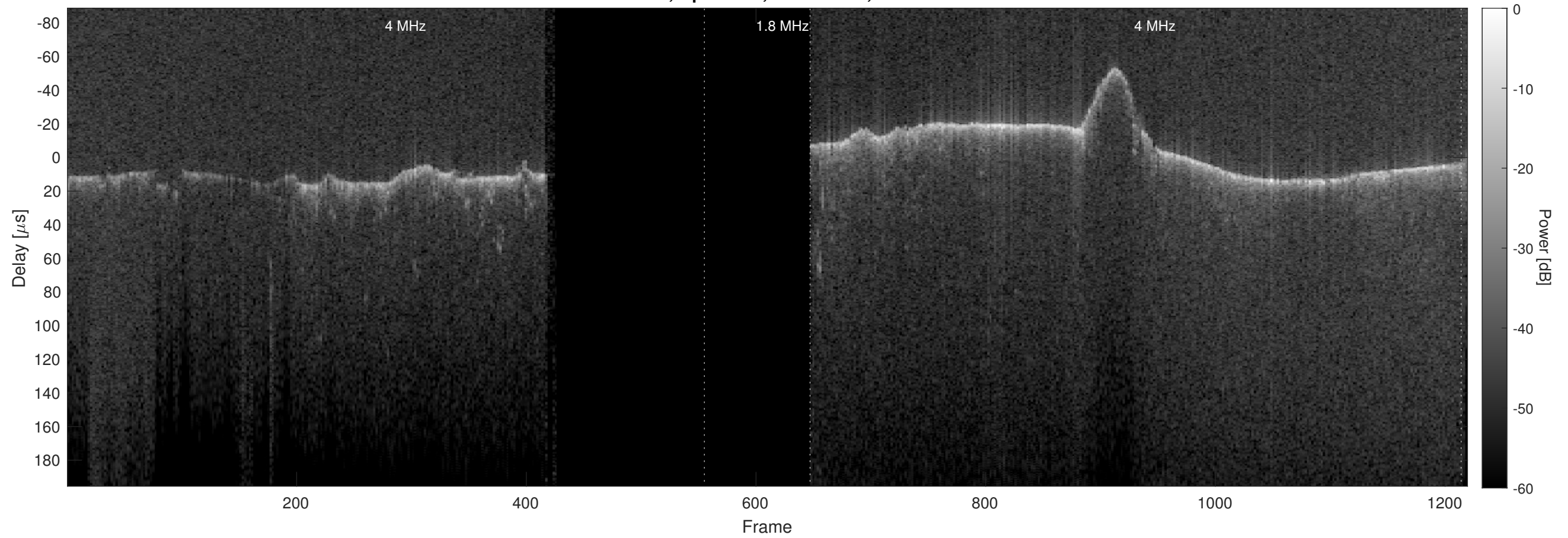
Orbit 23021, Optimized, No Window, Channel 2
