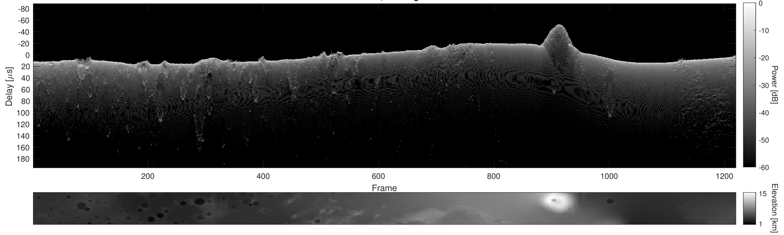
Orbit 23021, Cluttergram
