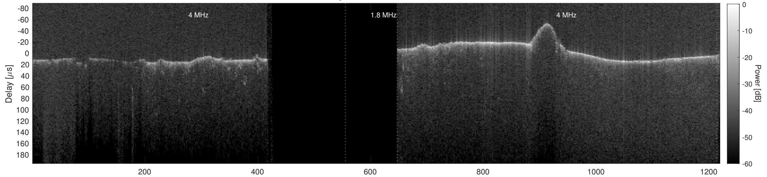
Orbit 23021, Cluttergram
