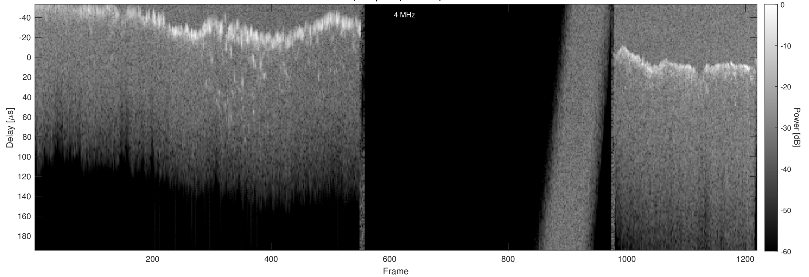
Orbit 23023, Chapman, Window, Channel 2
