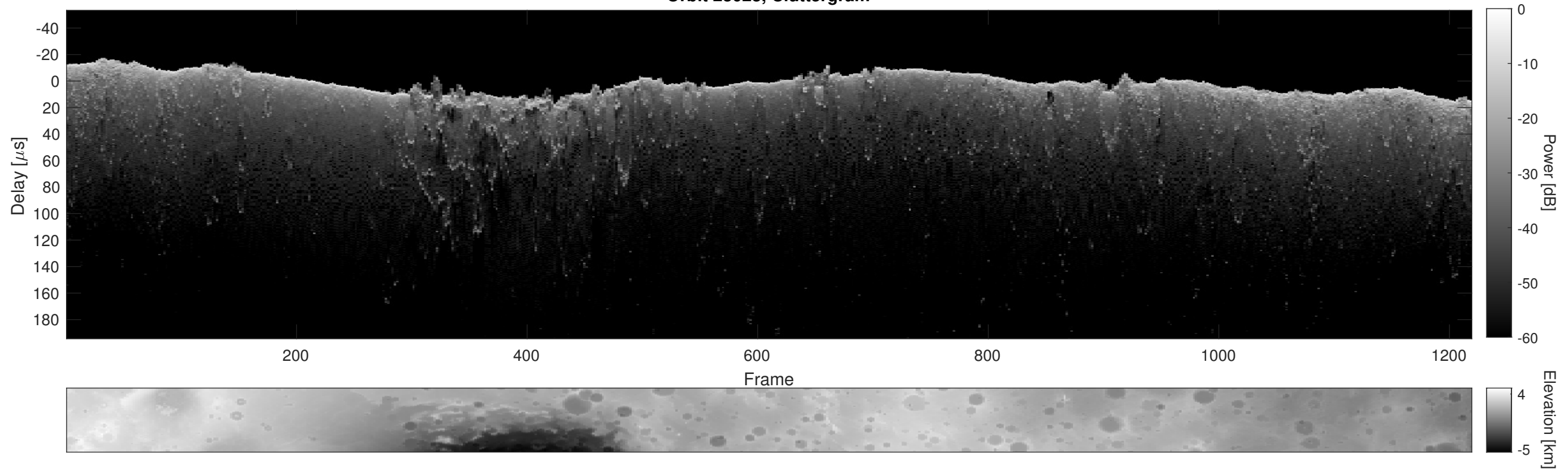
Orbit 23023, Cluttergram
