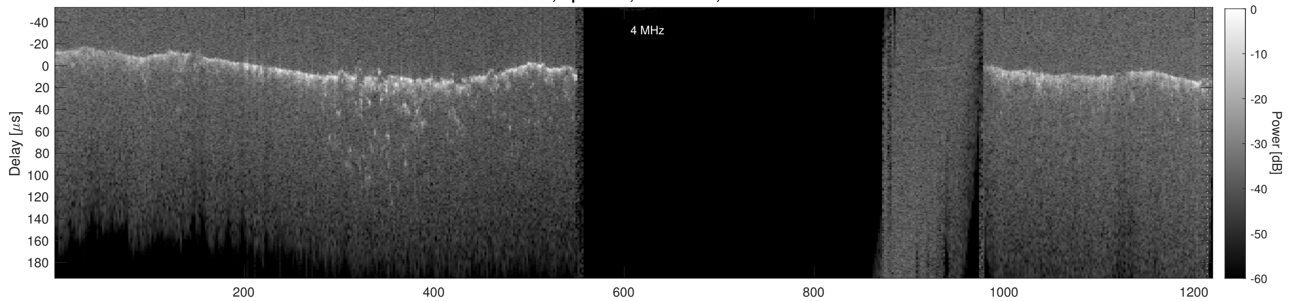
Orbit 23023, Cluttergram
