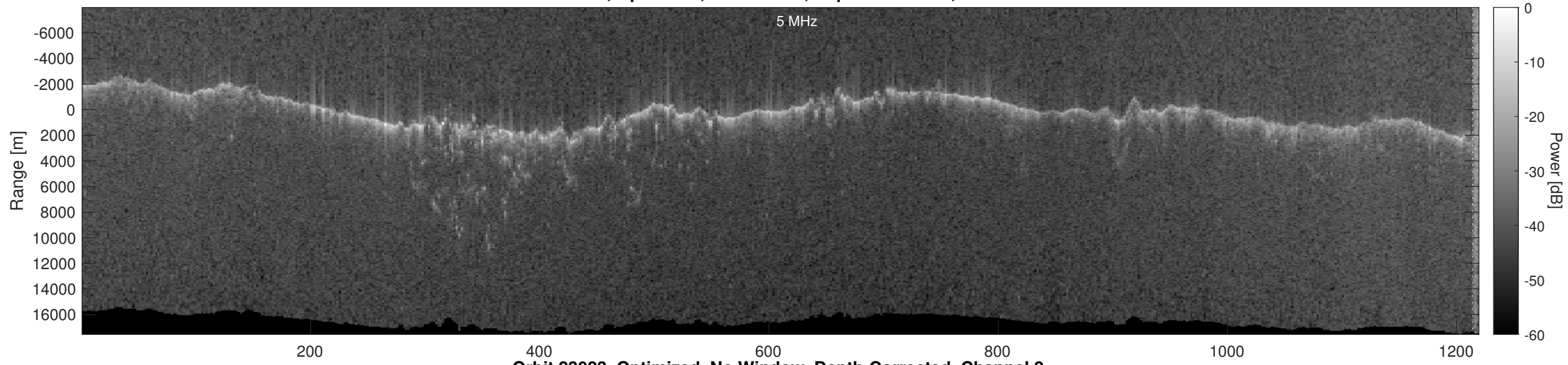
Orbit 23023, Optimized, No Window, Depth-Corrected, Channel 2
