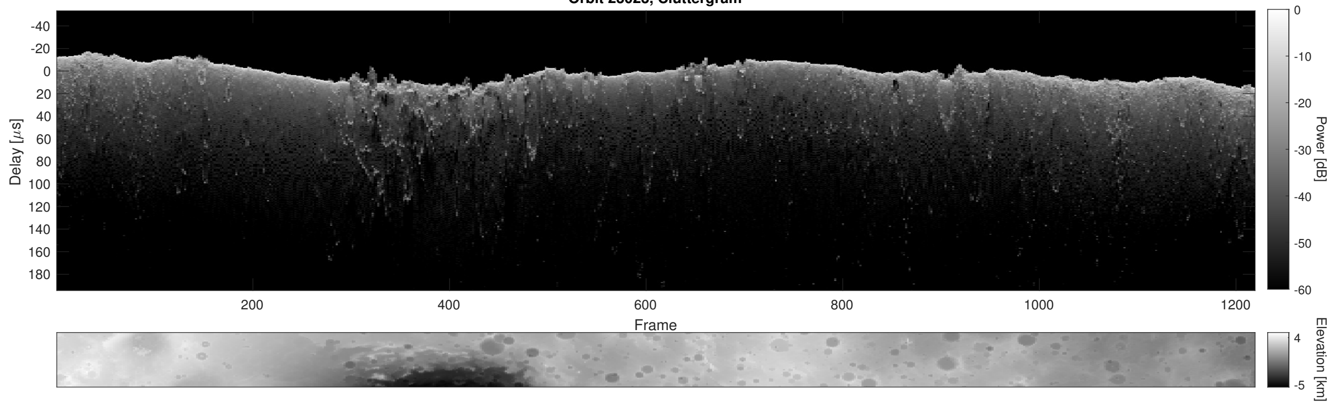
Orbit 23023, Cluttergram
