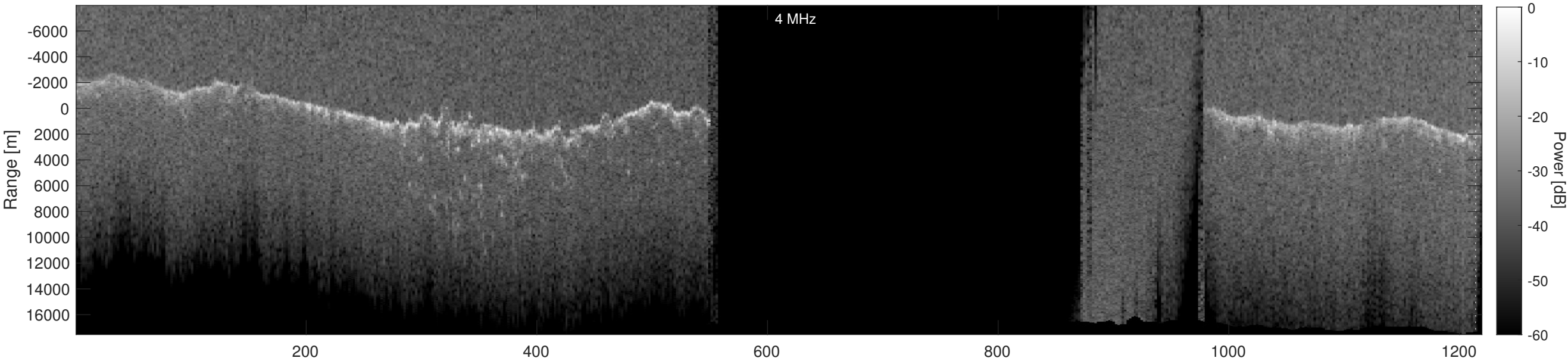
Orbit 23023, Depth-Corrected Cluttergram
