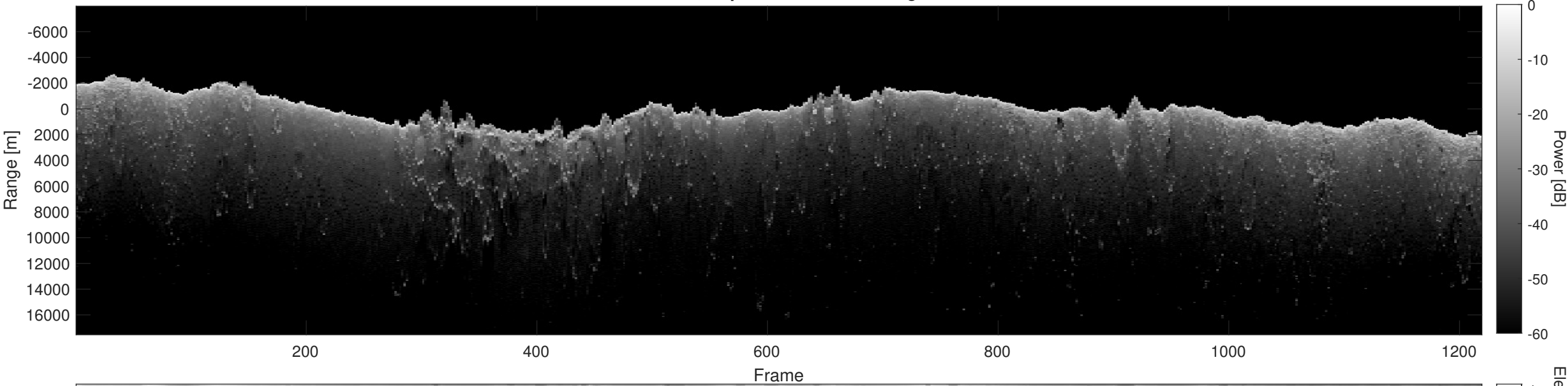
Orbit 23023, Depth-Corrected Cluttergram
