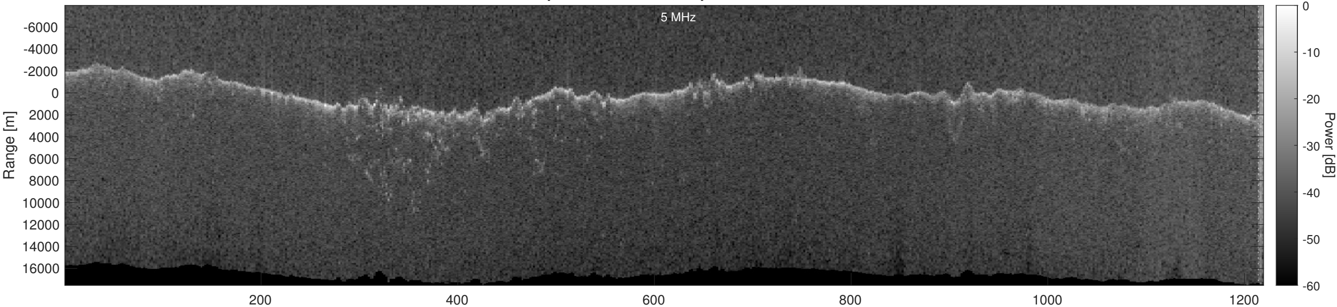
Orbit 23023, Optimized, Window, Depth-Corrected, Channel 2
