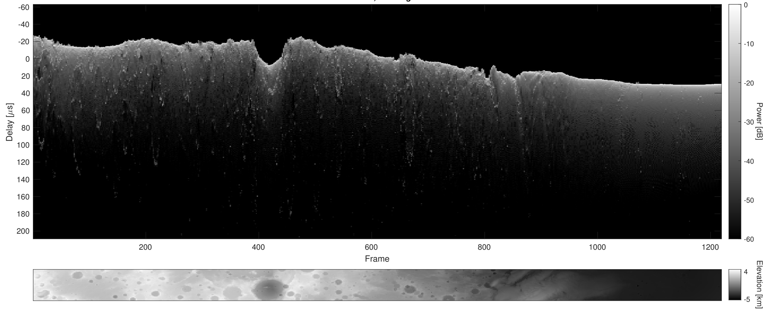
Orbit 23025, Cluttergram
