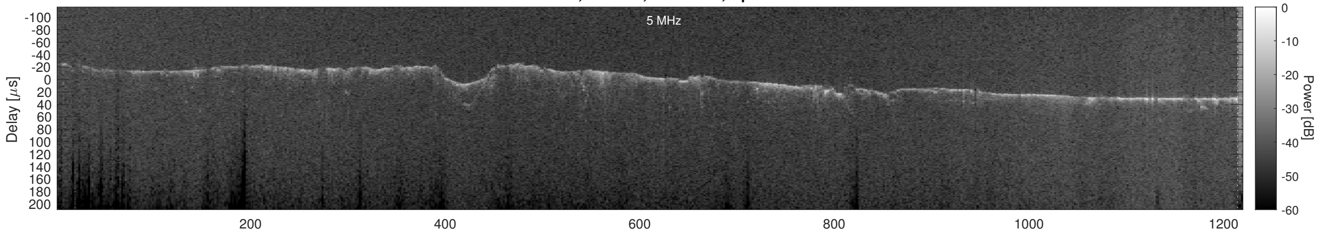
Orbit 23025, Cluttergram
