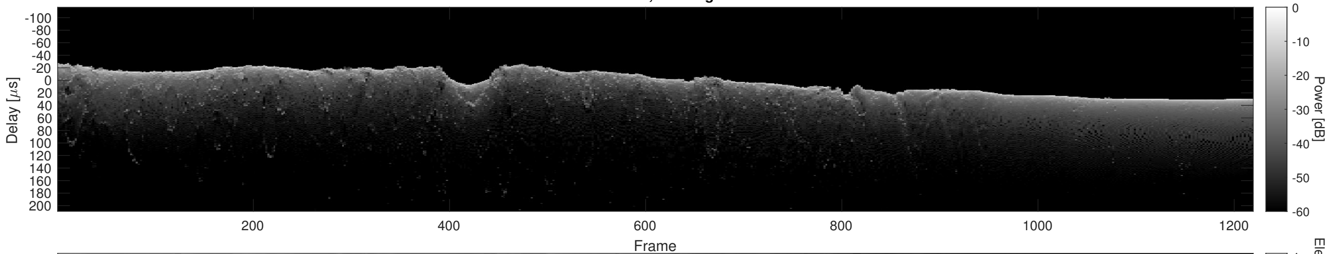
Orbit 23025, Cluttergram
