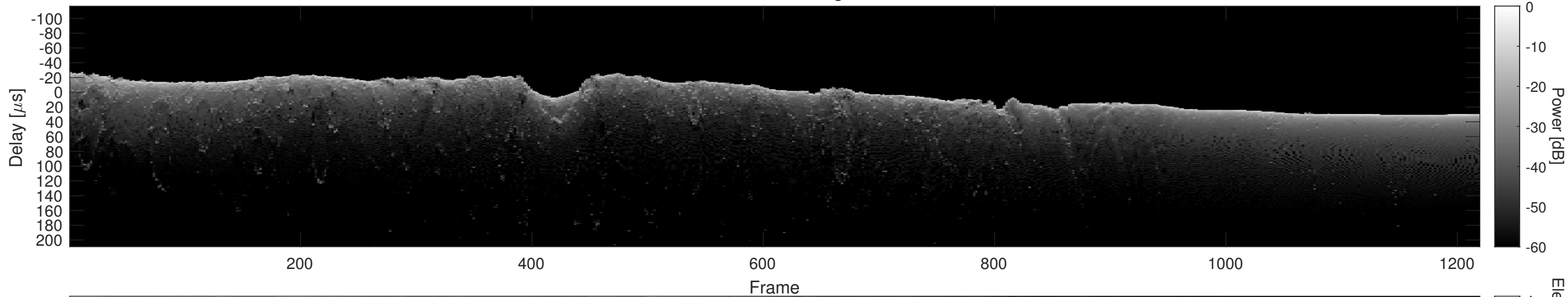
Orbit 23025, Cluttergram
