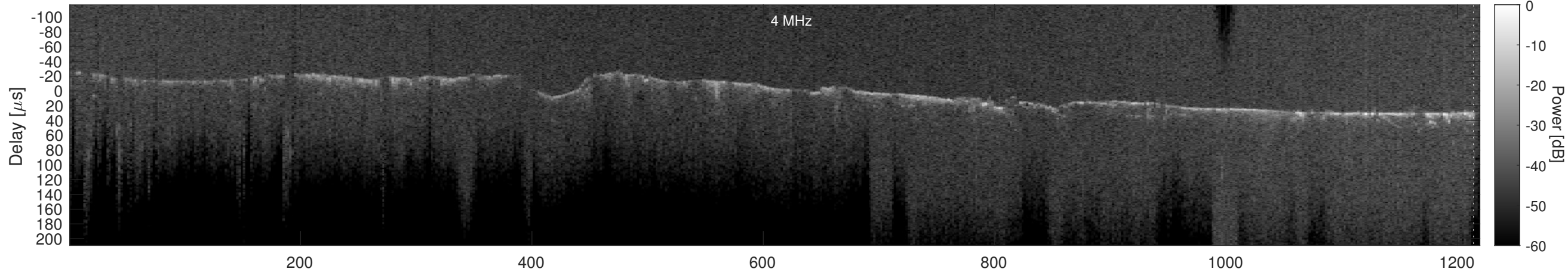
Orbit 23025, Cluttergram
