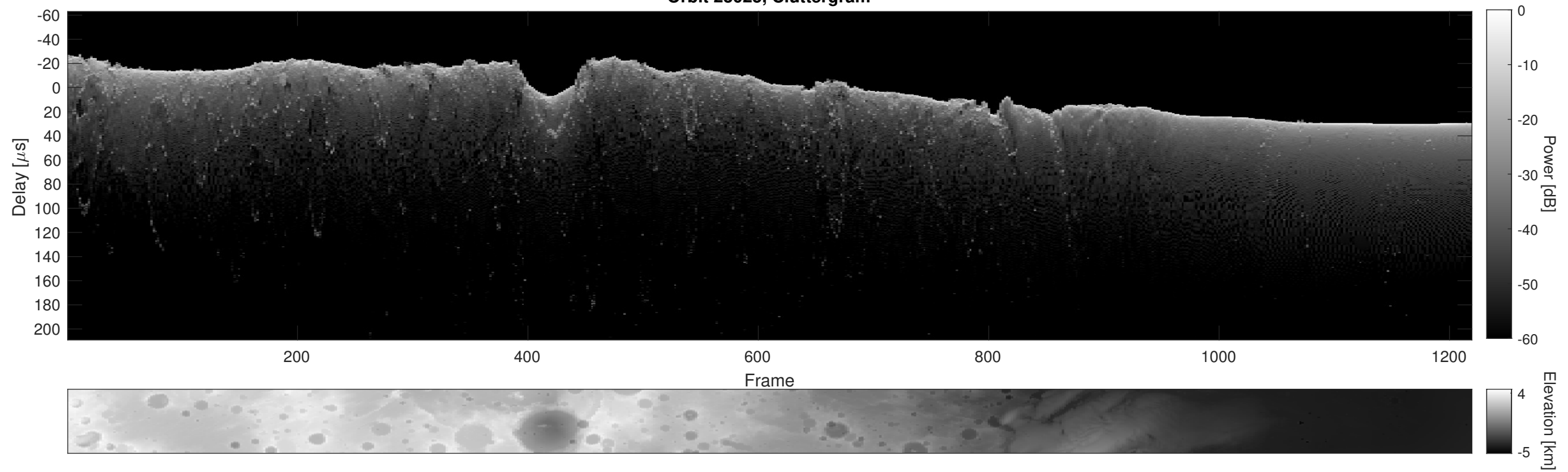
Orbit 23025, Cluttergram
