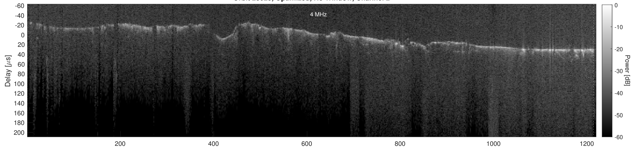
Orbit 23025, Cluttergram
