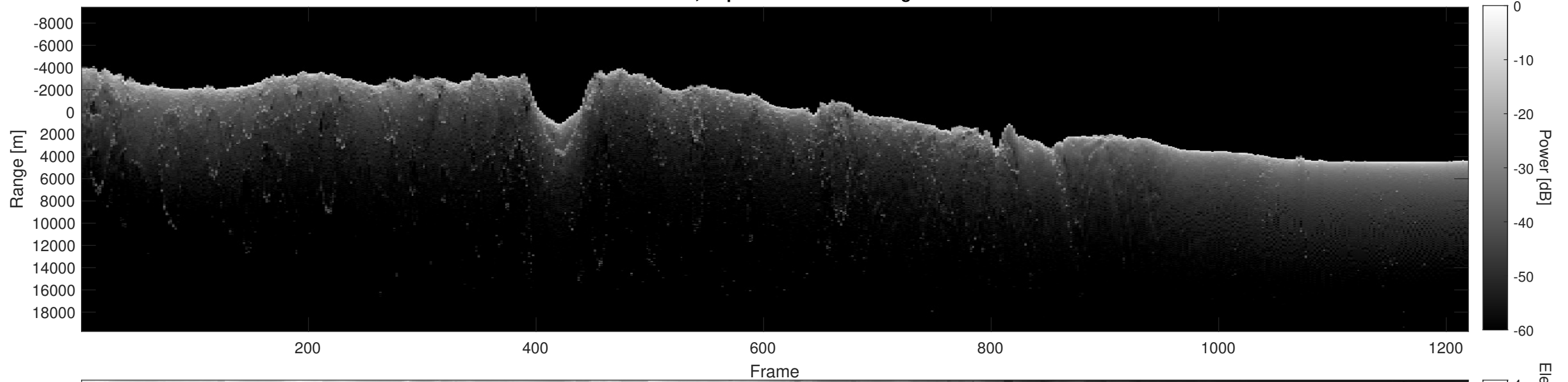
Orbit 23025, Depth-Corrected Cluttergram
