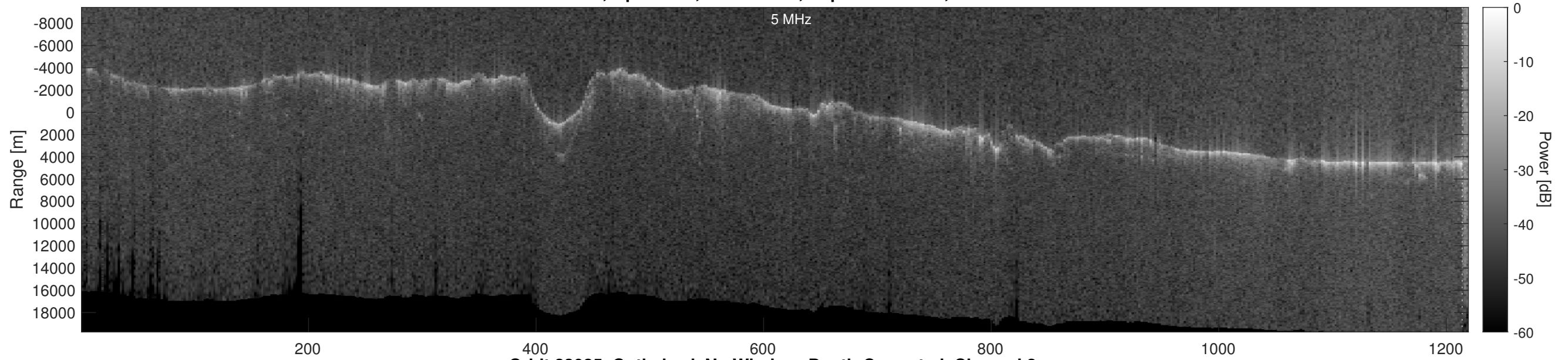
Orbit 23025, Optimized, No Window, Depth-Corrected, Channel 2
