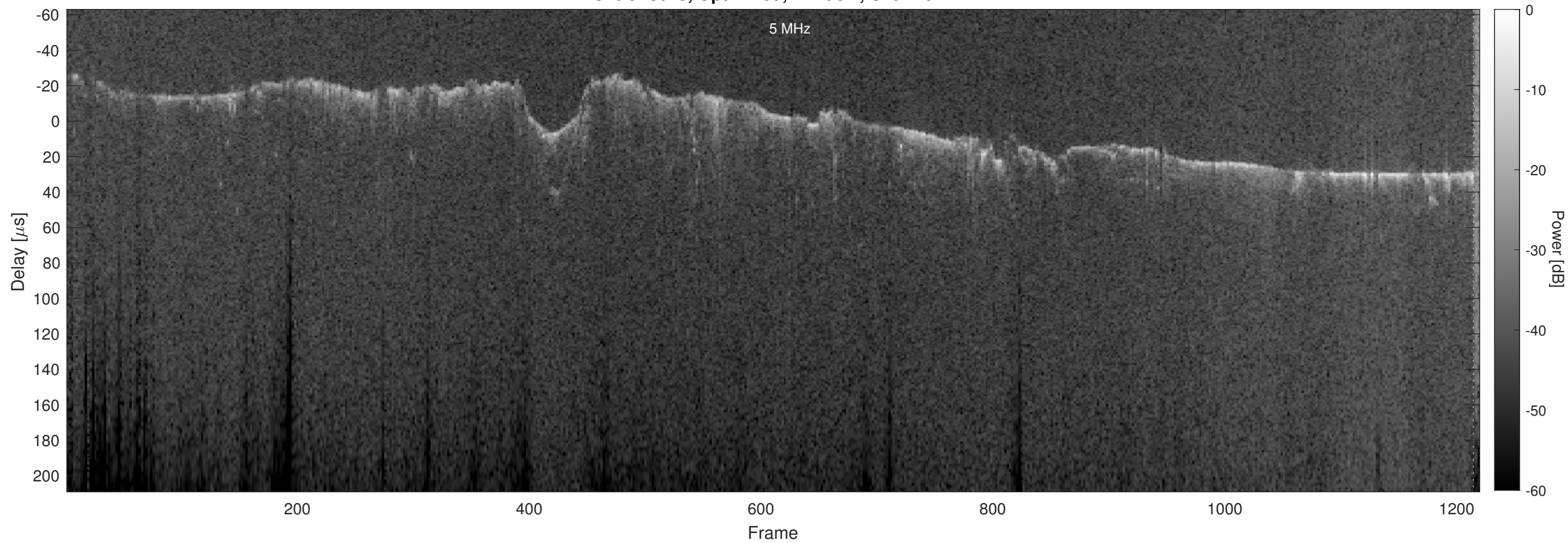
Orbit 23025, Optimized, Window, Channel 2
