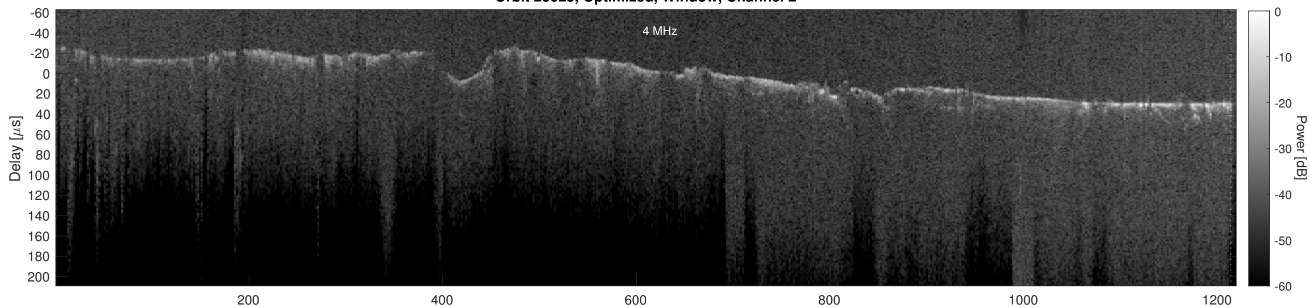
Orbit 23025, Cluttergram
