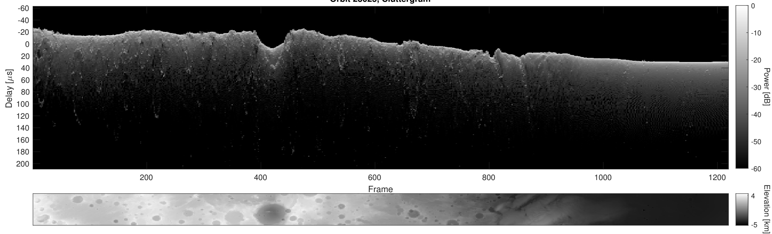
Orbit 23025, Cluttergram
