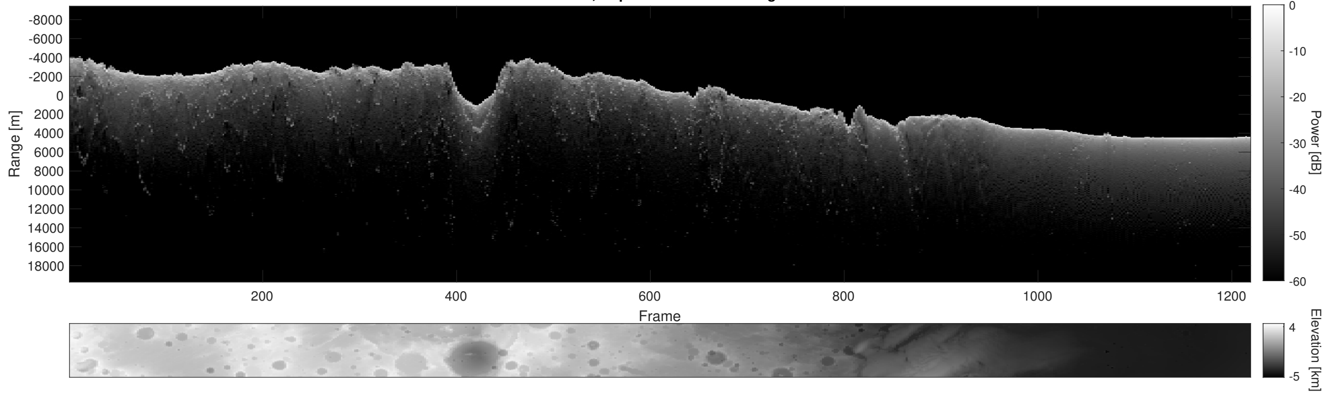
Orbit 23025, Depth-Corrected Cluttergram
