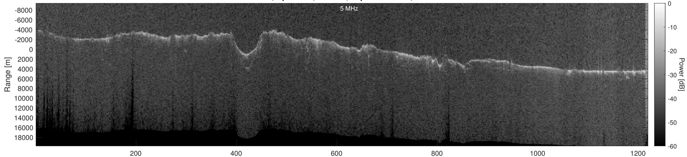
Orbit 23025, Optimized, Window, Depth-Corrected, Channel 2
