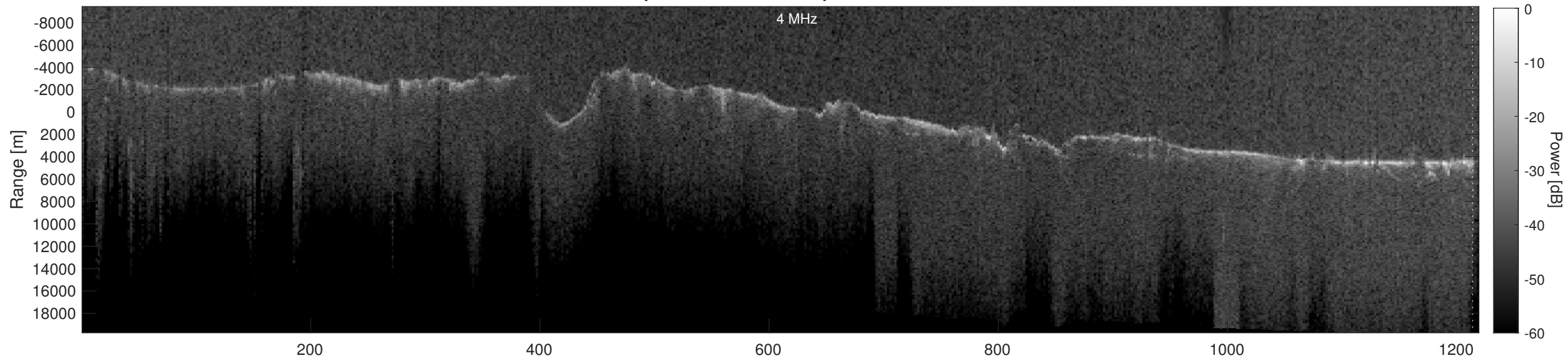
Orbit 23025, Depth-Corrected Cluttergram
