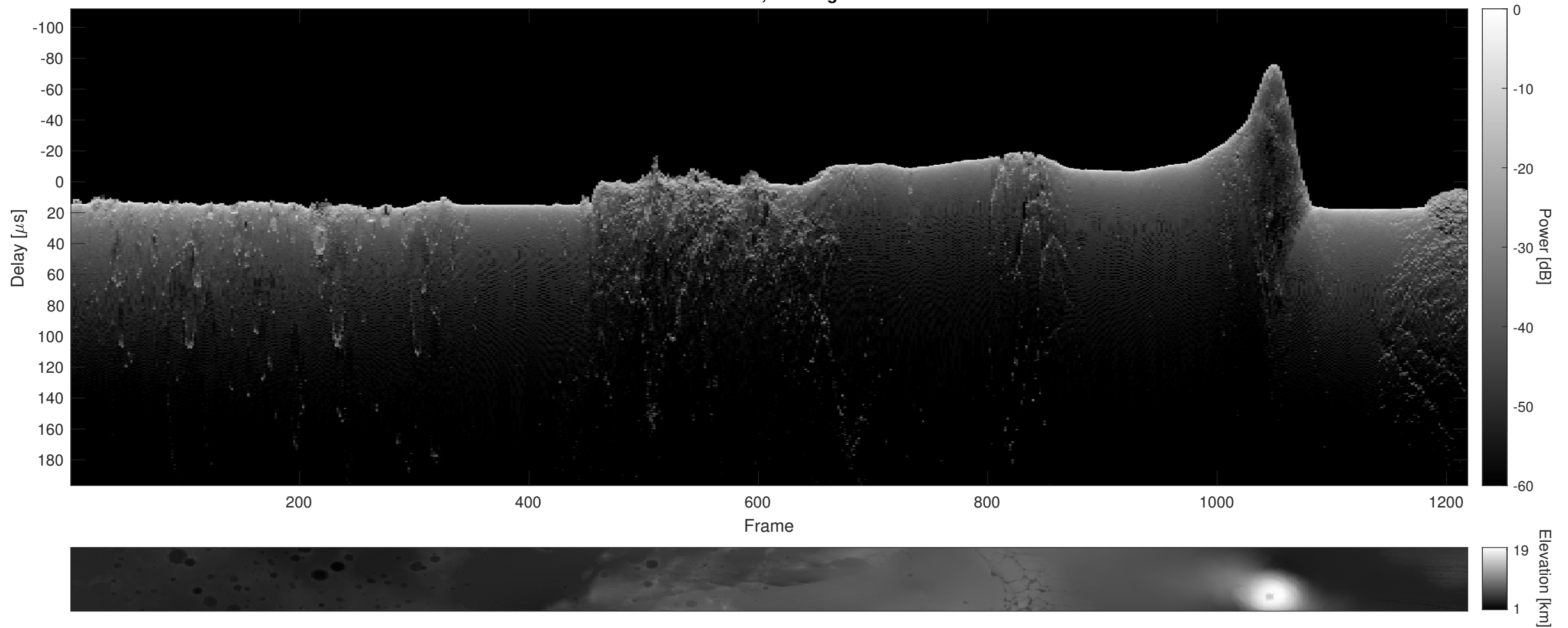
Orbit 23028, Cluttergram
