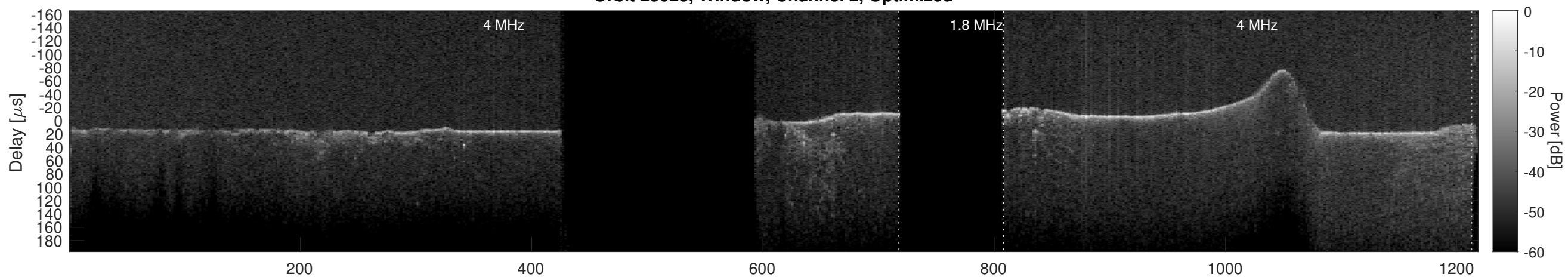
Orbit 23028, Cluttergram
