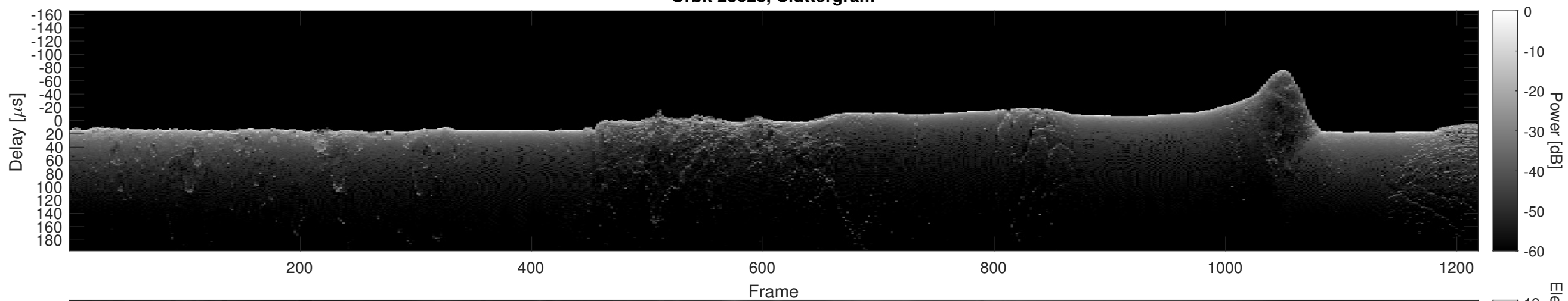
Orbit 23028, Cluttergram
