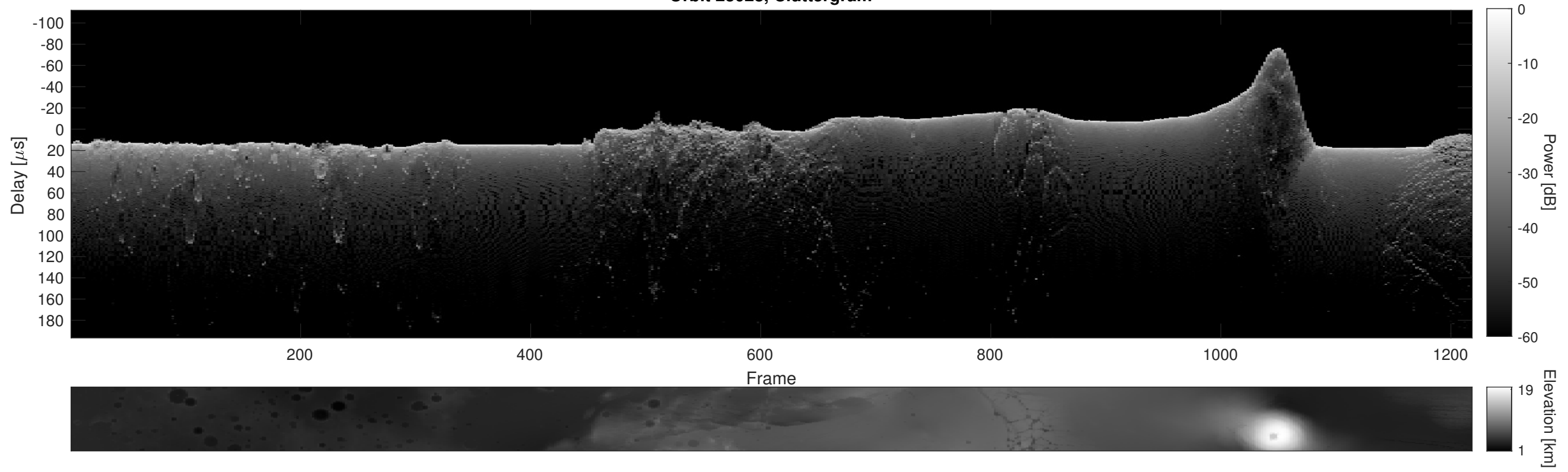
Orbit 23028, Cluttergram
