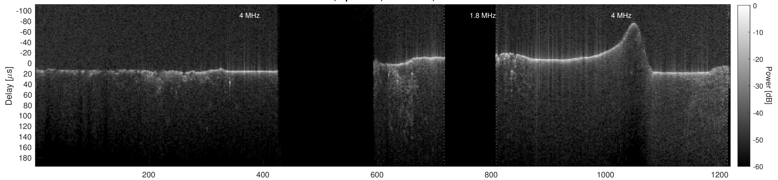
Orbit 23028, Cluttergram
