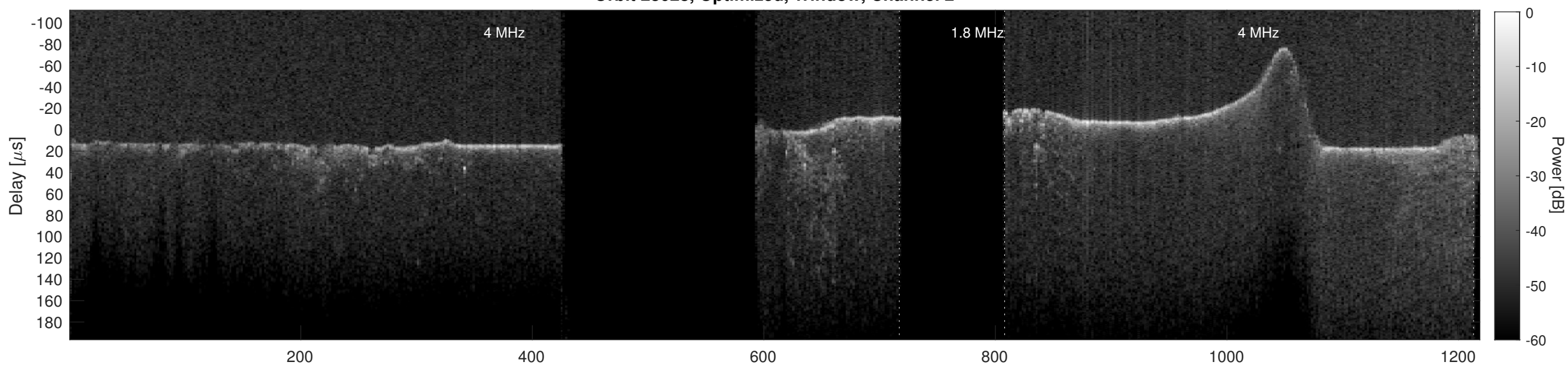
Orbit 23028, Cluttergram
