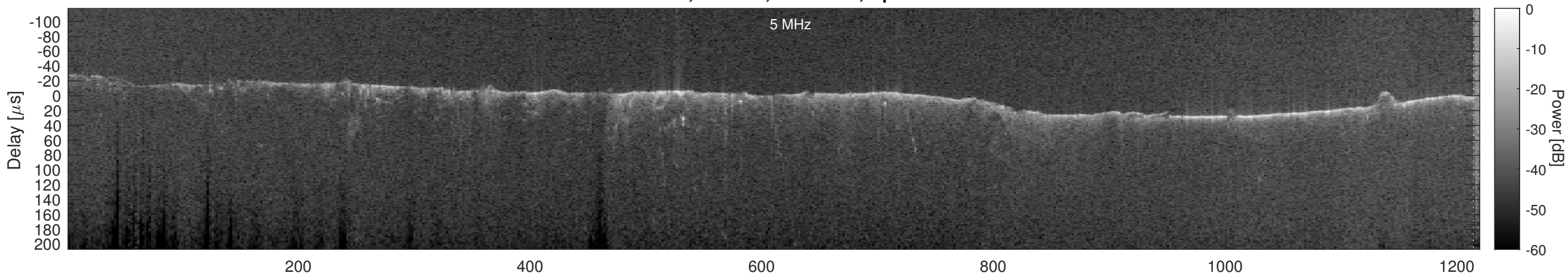
Orbit 23029, Cluttergram
