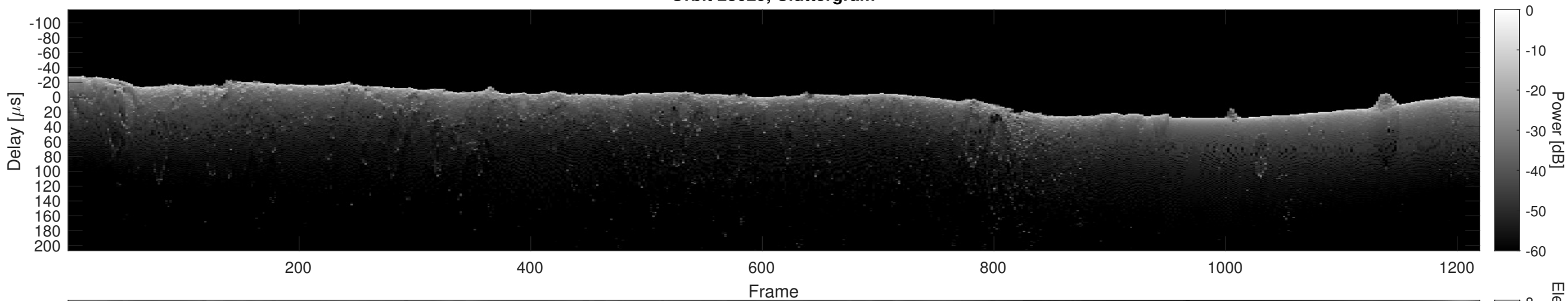
Orbit 23029, Cluttergram
