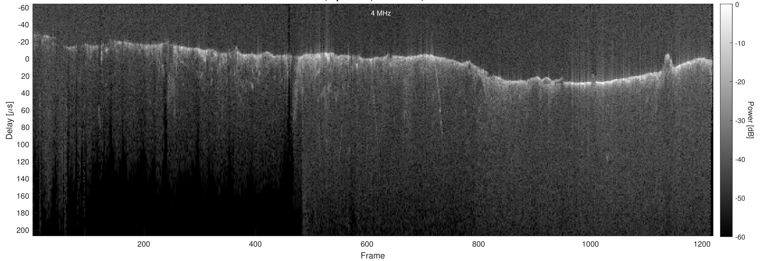
Orbit 23029, Optimized, No Window, Channel 2
