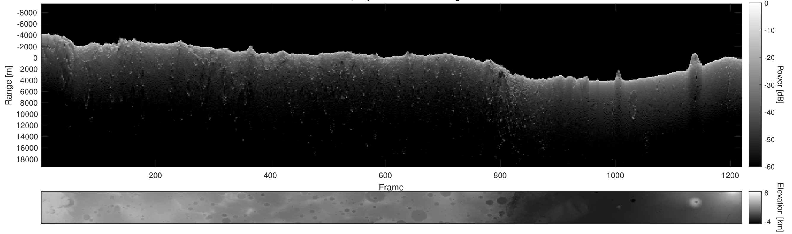
Orbit 23029, Depth-Corrected Cluttergram
