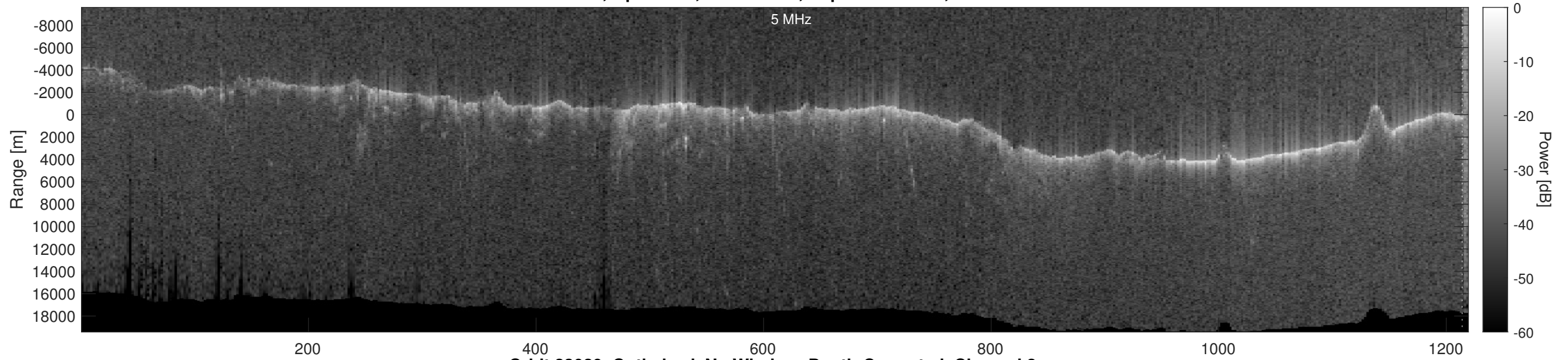
Orbit 23029, Optimized, No Window, Depth-Corrected, Channel 2
