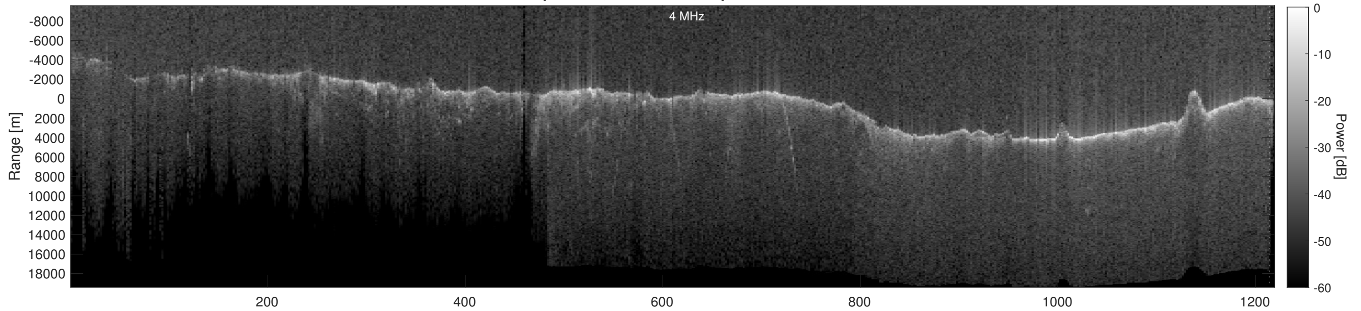
Orbit 23029, Depth-Corrected Cluttergram
