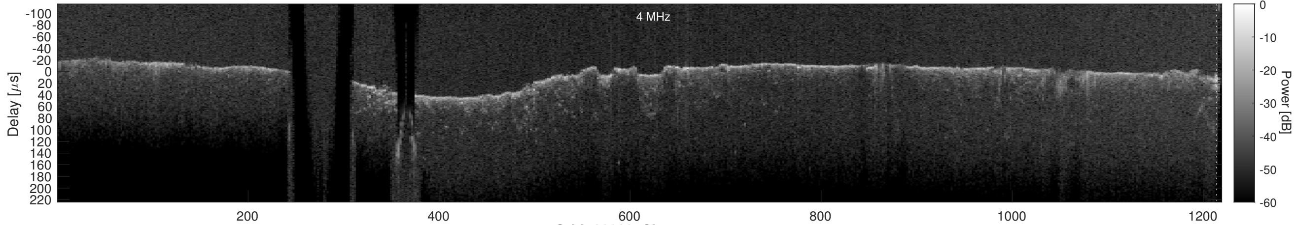
Orbit 23030, Cluttergram
