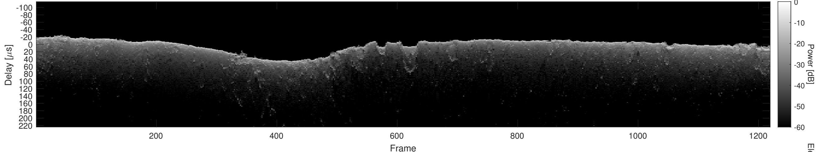
Orbit 23030, Cluttergram
