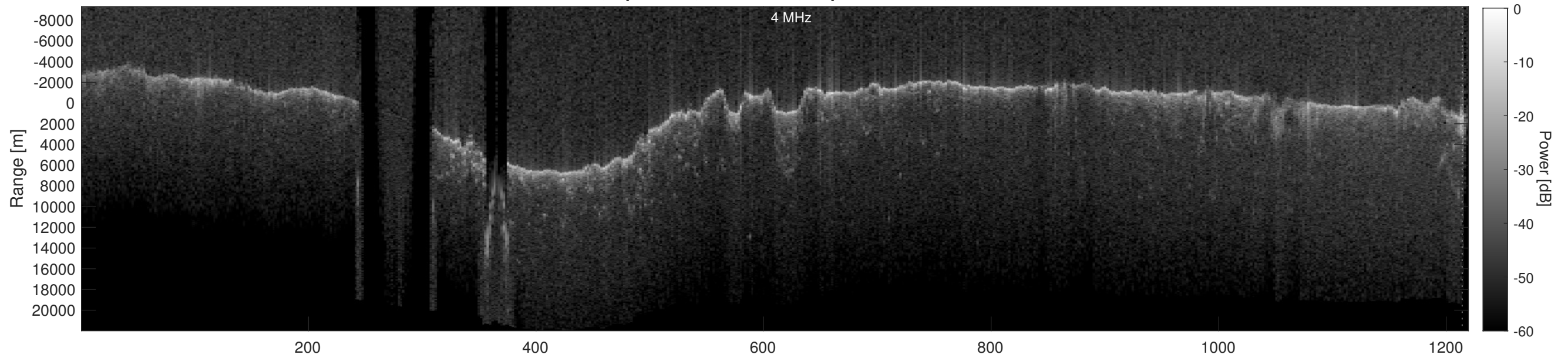
Orbit 23030, Depth-Corrected Cluttergram
