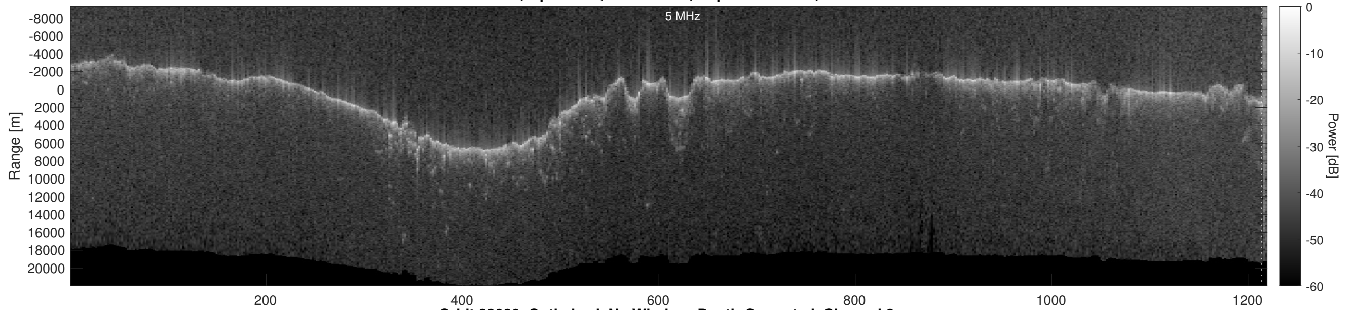
Orbit 23030, Optimized, No Window, Depth-Corrected, Channel 2
