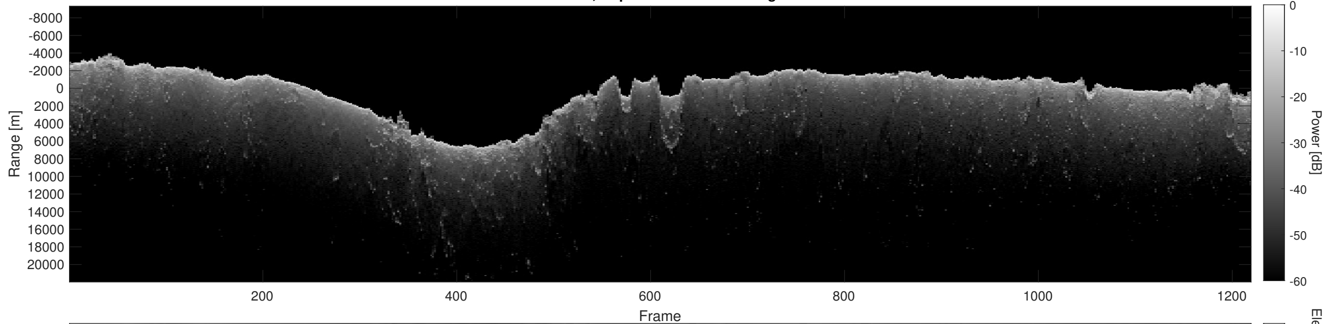
Orbit 23030, Depth-Corrected Cluttergram
