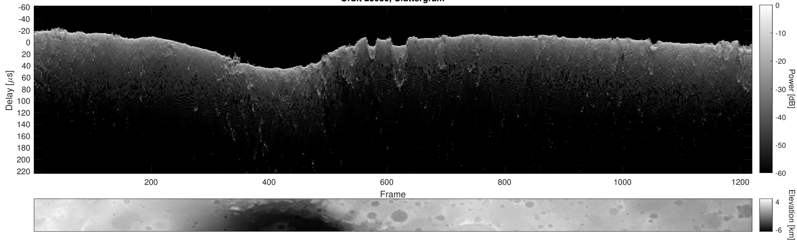
Orbit 23030, Cluttergram
