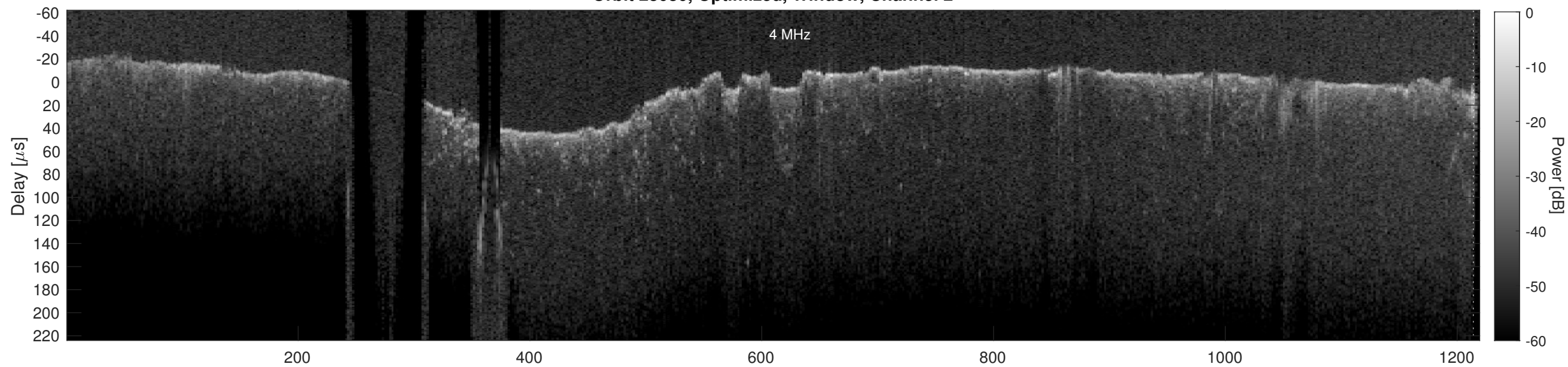
Orbit 23030, Cluttergram
