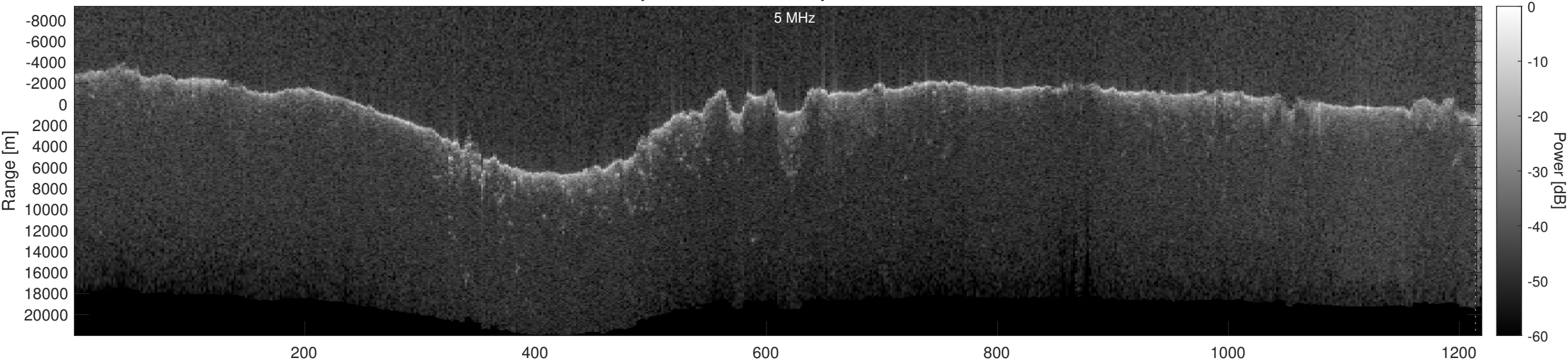
Orbit 23030, Optimized, Window, Depth-Corrected, Channel 2
