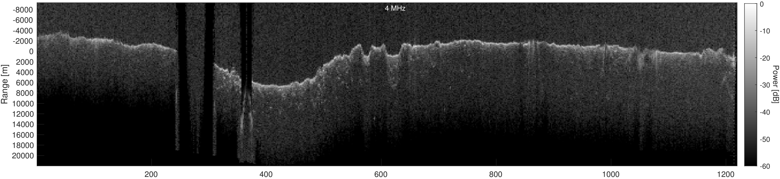
Orbit 23030, Depth-Corrected Cluttergram
