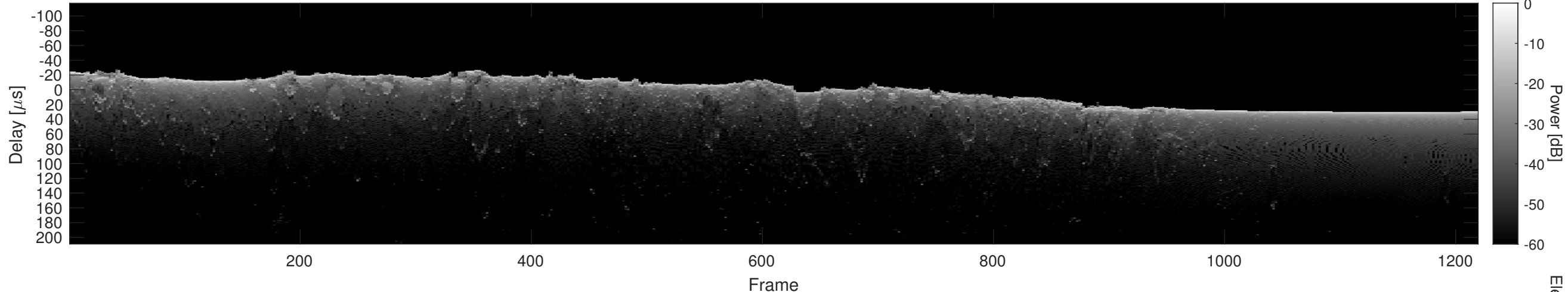
Orbit 23032, Cluttergram
