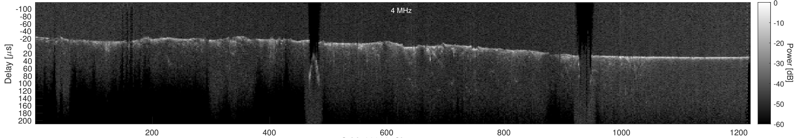
Orbit 23032, Cluttergram
