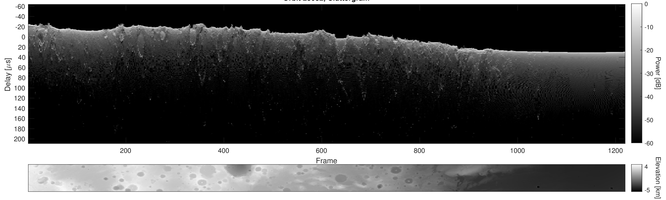
Orbit 23032, Cluttergram
