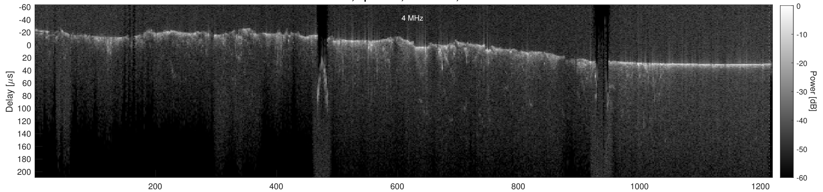
Orbit 23032, Cluttergram
