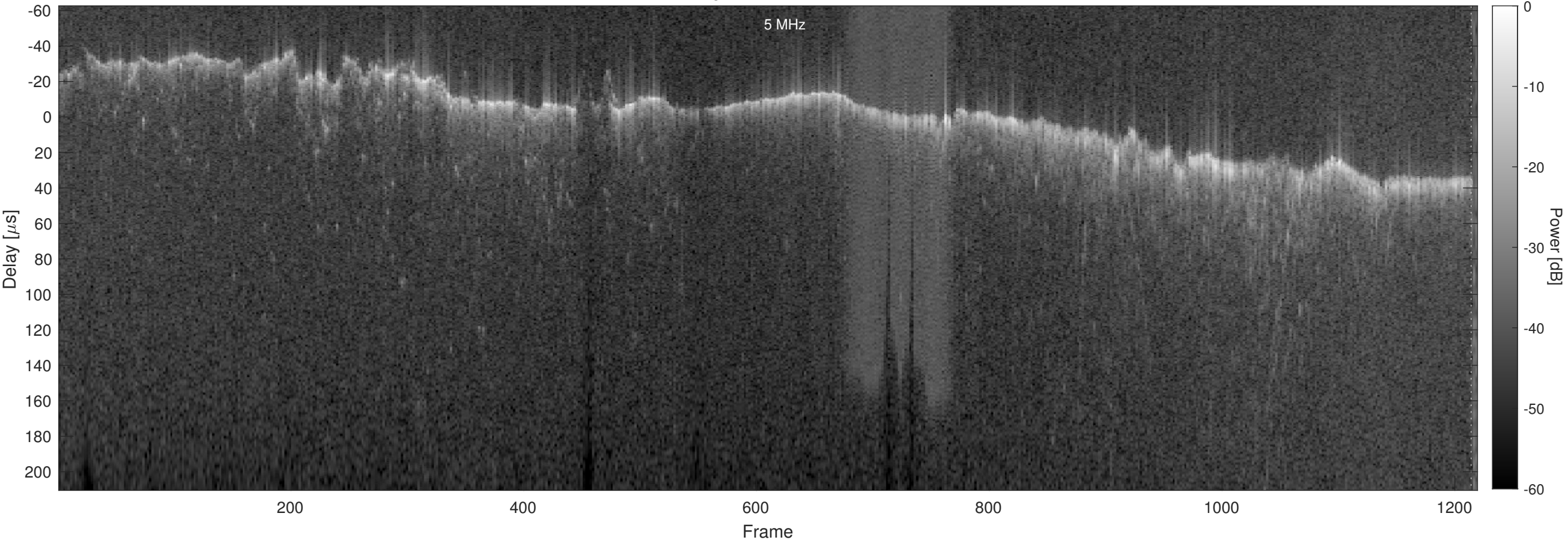
Orbit 23033, Chapman, No Window, Channel 2
