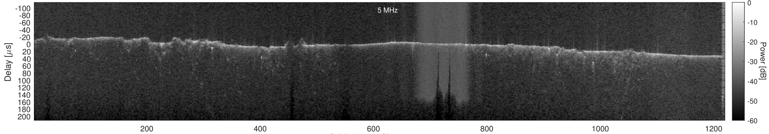
Orbit 23033, Cluttergram
