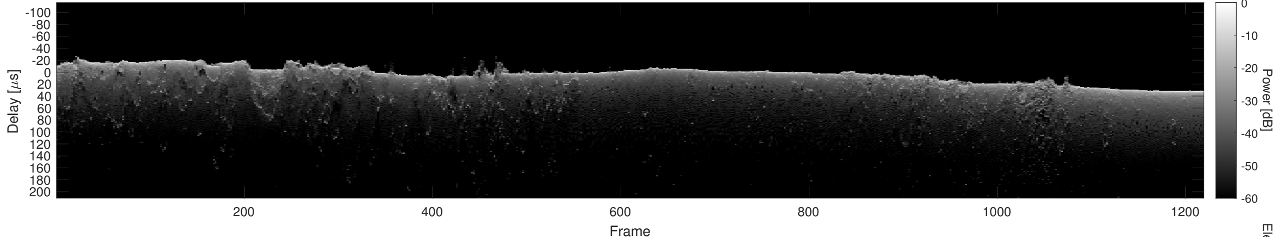
Orbit 23033, Cluttergram
