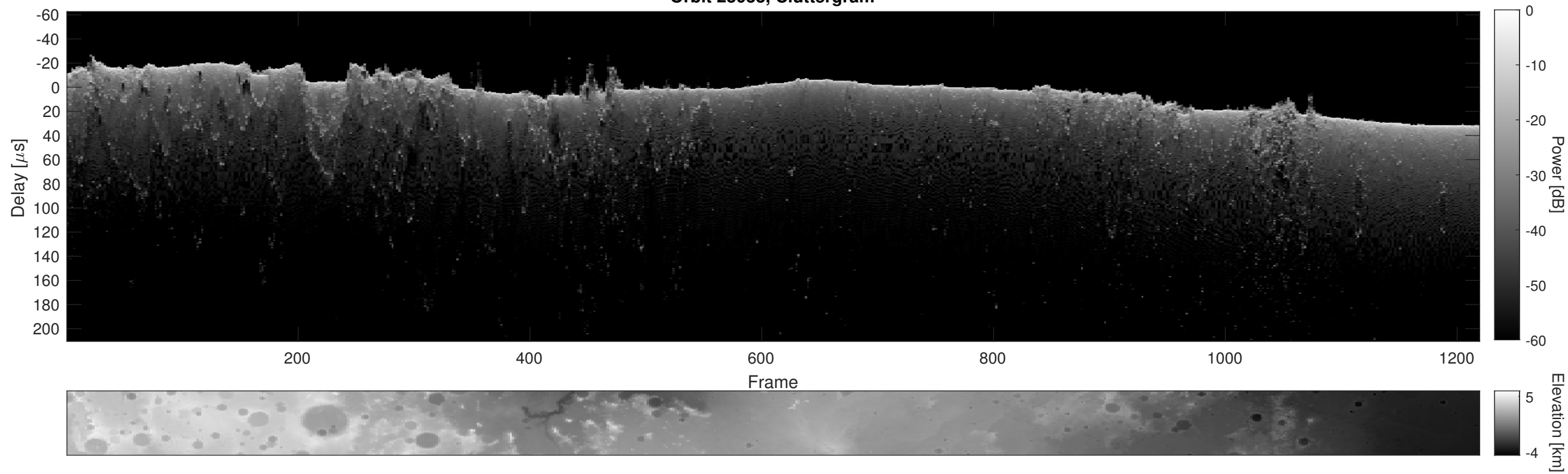
Orbit 23033, Cluttergram
