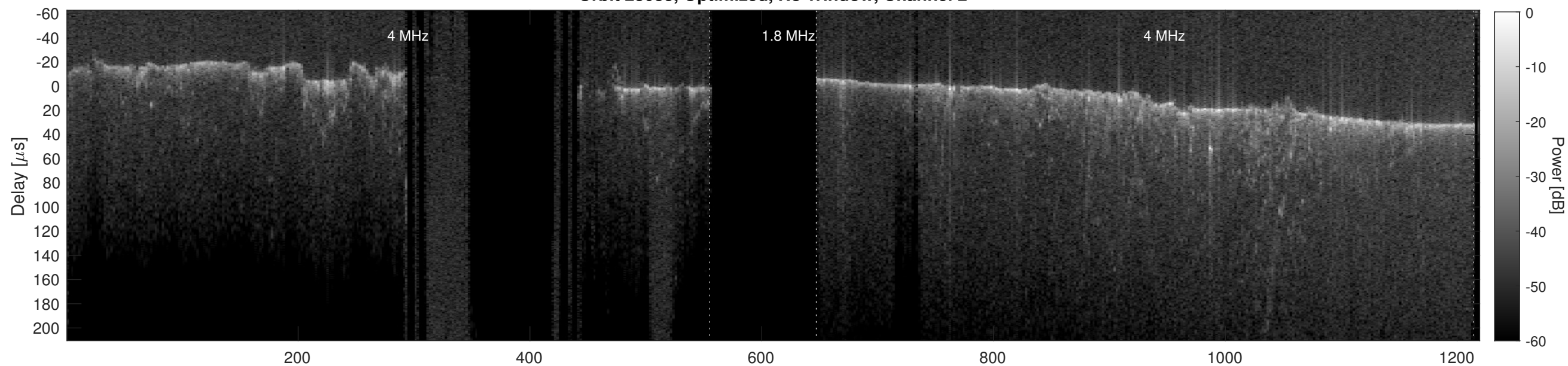
Orbit 23033, Cluttergram
