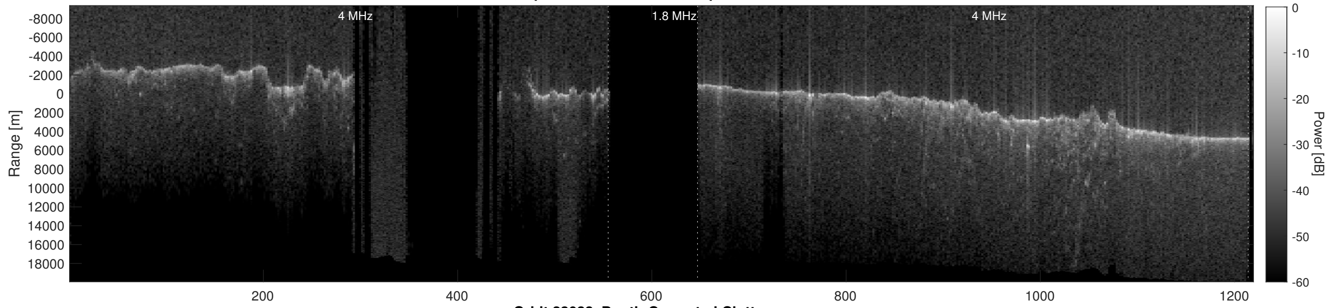
Orbit 23033, Depth-Corrected Cluttergram
