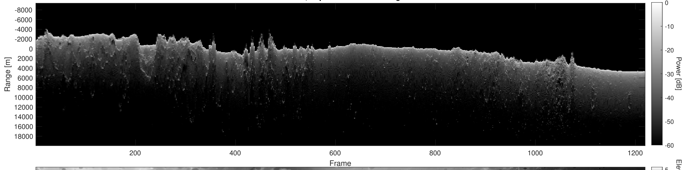
Orbit 23033, Depth-Corrected Cluttergram
