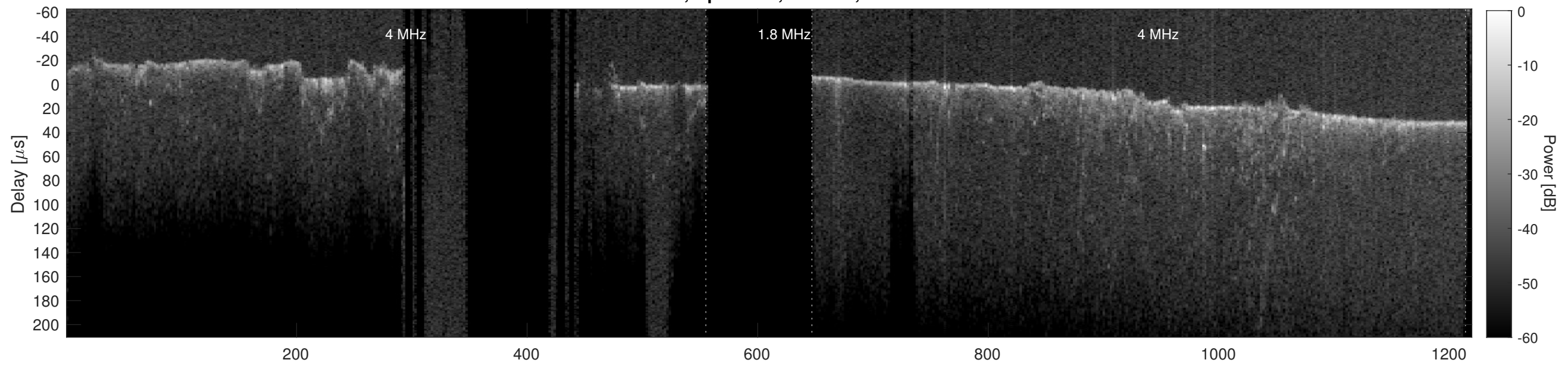
Orbit 23033, Cluttergram
