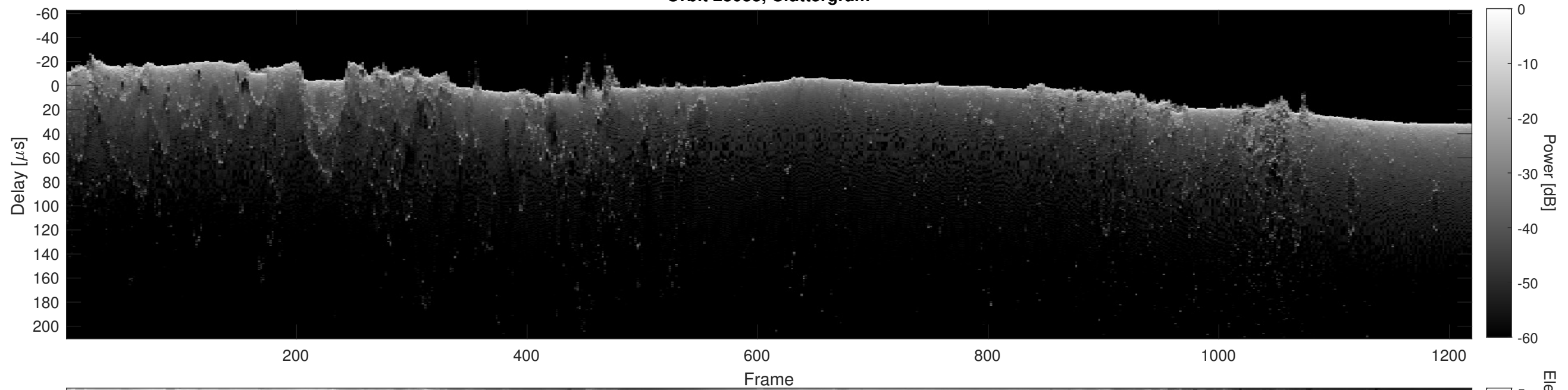
Orbit 23033, Cluttergram
