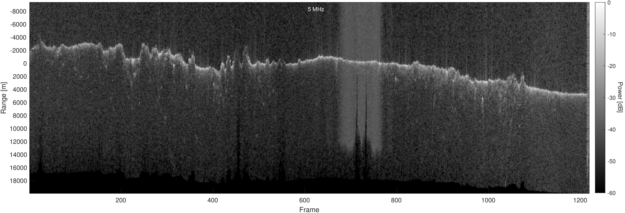
Orbit 23033, Optimized, Window, Depth-Corrected, Channel 2
