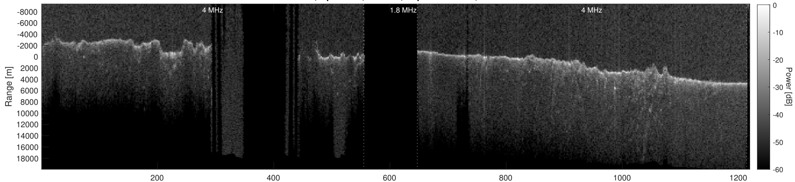
Orbit 23033, Depth-Corrected Cluttergram
