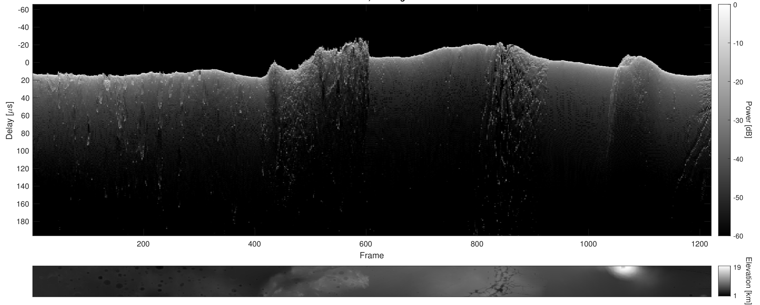
Orbit 23035, Cluttergram
