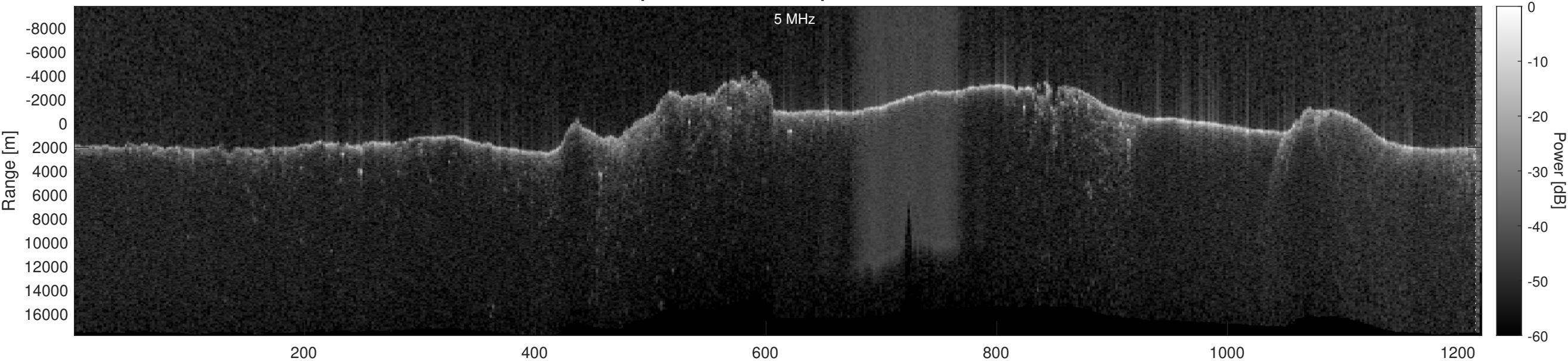
Orbit 23035, Optimized, Window, Depth-Corrected, Channel 2
