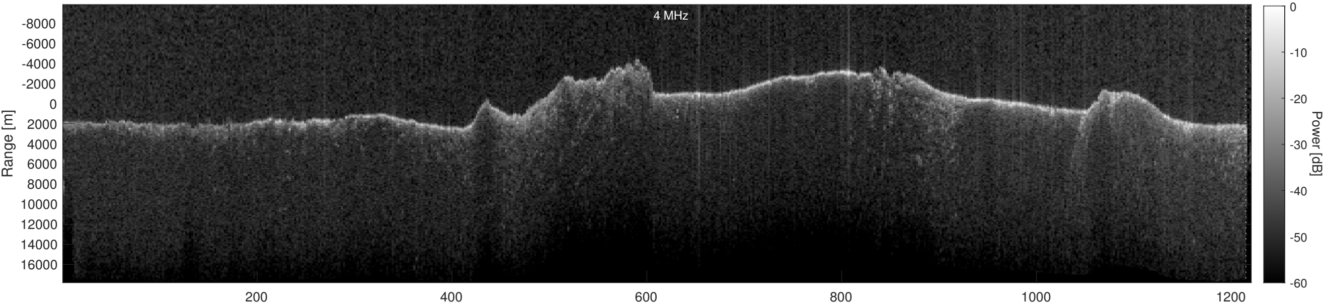
Orbit 23035, Depth-Corrected Cluttergram
