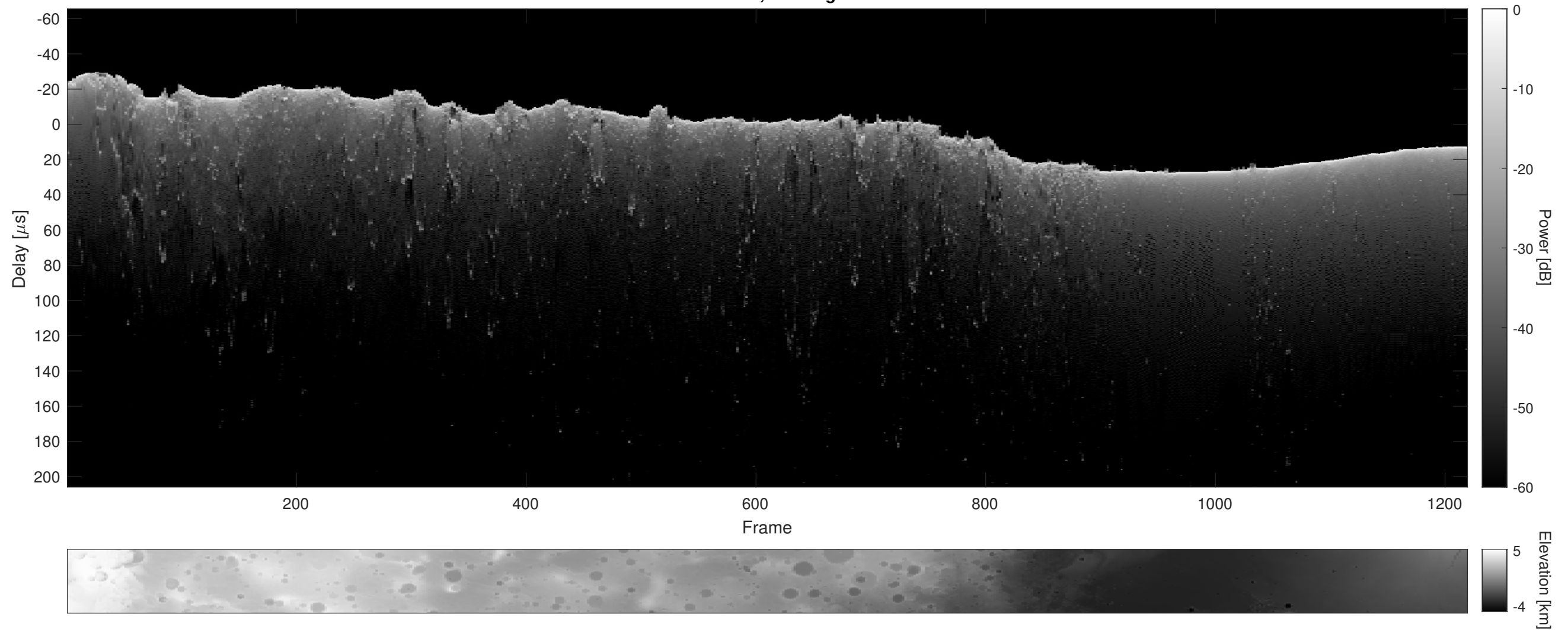
Orbit 23036, Cluttergram
