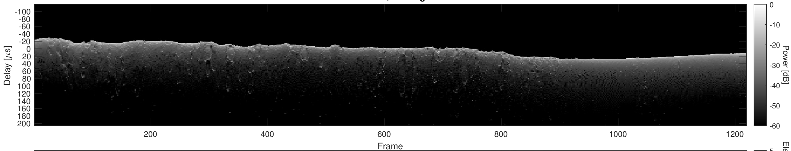
Orbit 23036, Cluttergram
