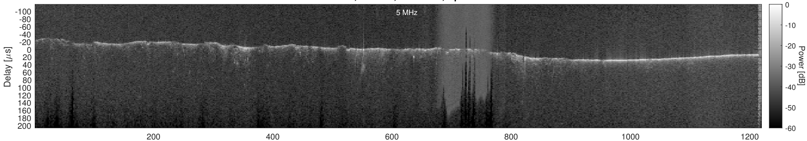
Orbit 23036, Cluttergram
