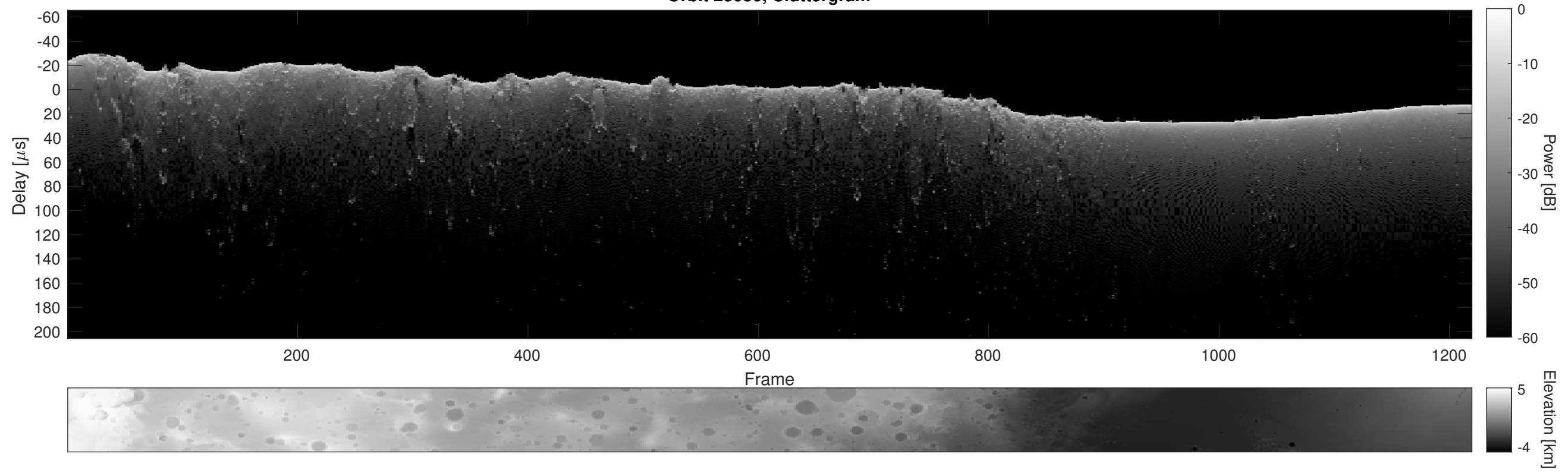
Orbit 23036, Cluttergram
