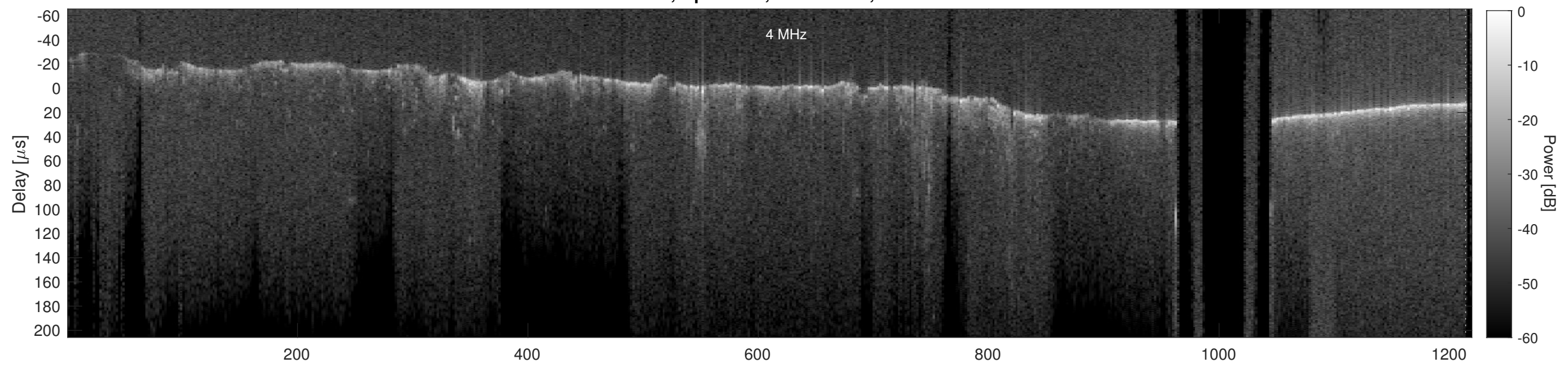
Orbit 23036, Cluttergram
