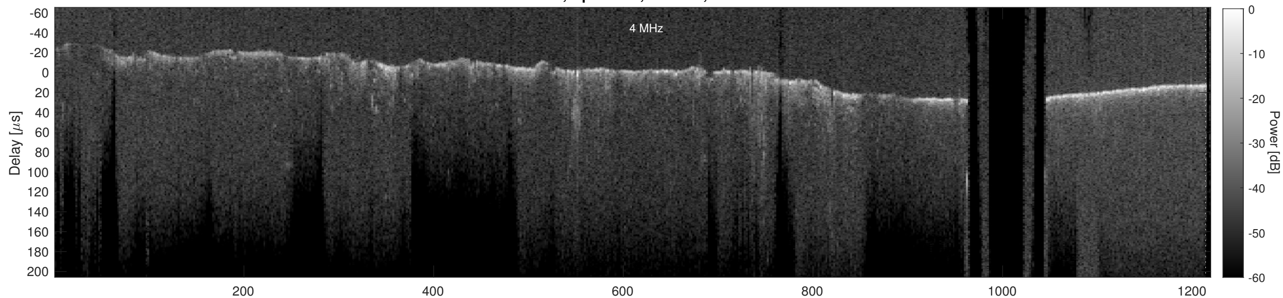
Orbit 23036, Cluttergram
