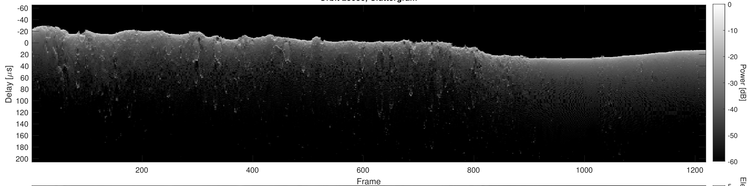
Orbit 23036, Cluttergram
