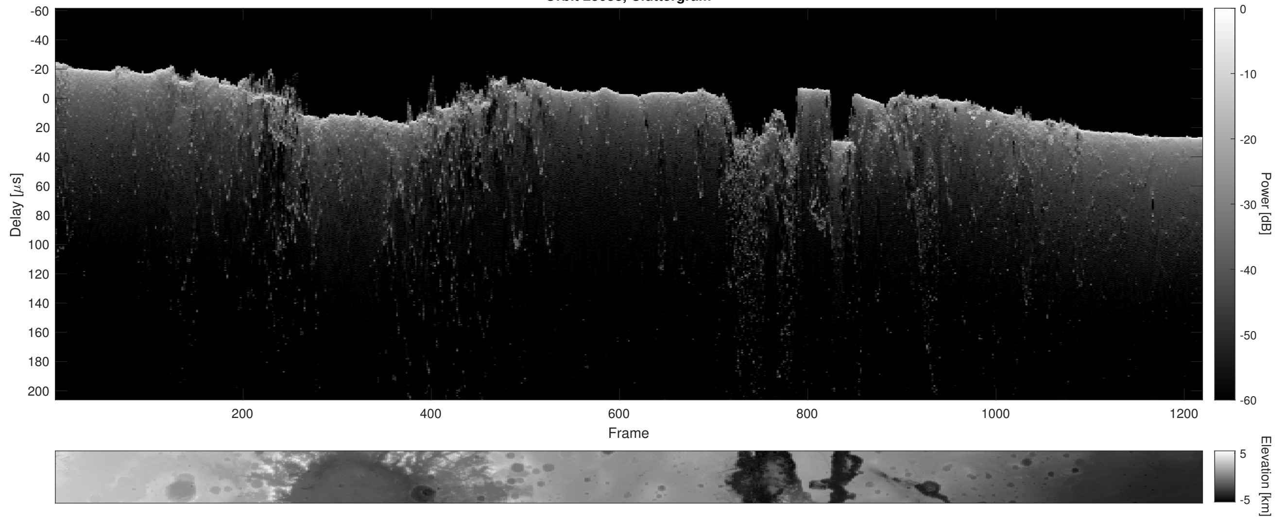
Orbit 23038, Cluttergram
