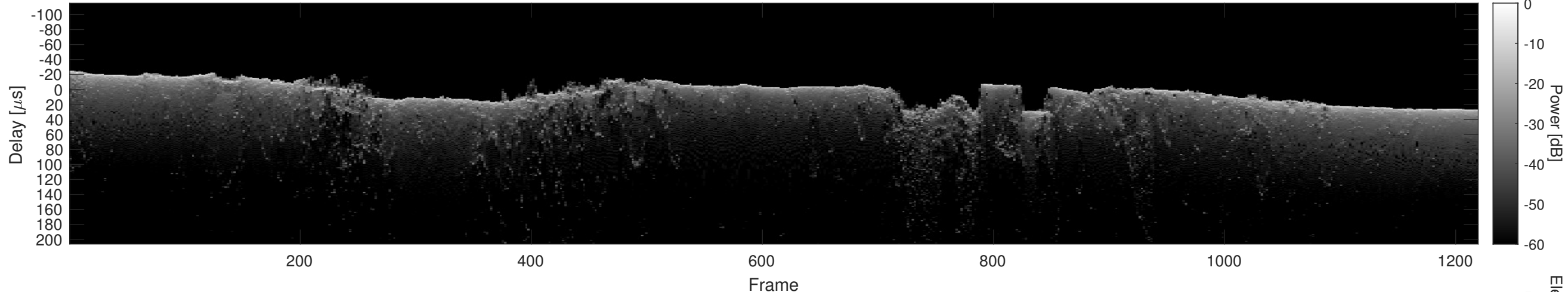
Orbit 23038, Cluttergram
