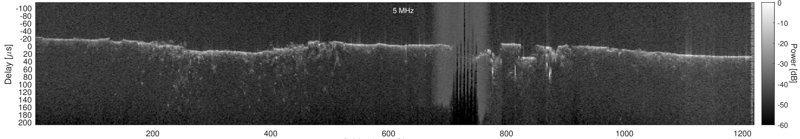
Orbit 23038, Cluttergram
