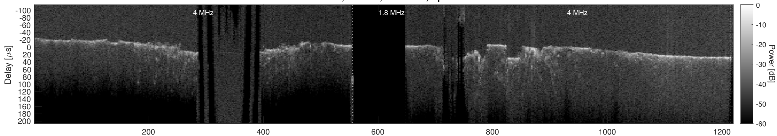
Orbit 23038, Cluttergram
