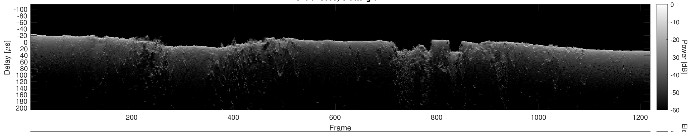
Orbit 23038, Cluttergram
