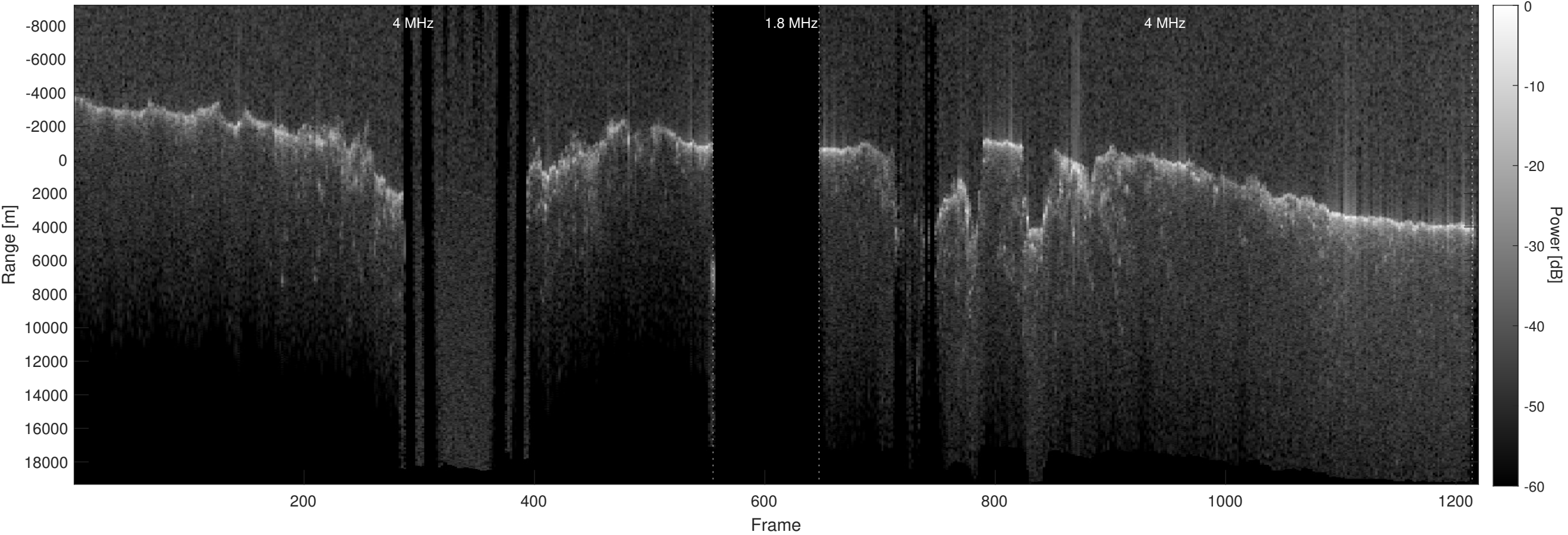
Orbit 23038, Optimized, No Window, Depth-Corrected, Channel 2
