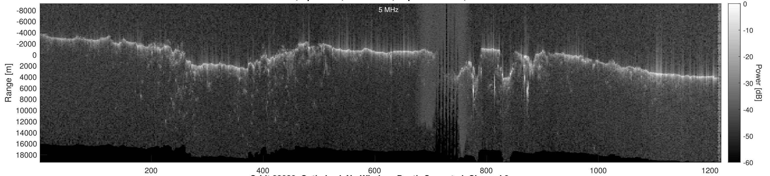
Orbit 23038, Optimized, No Window, Depth-Corrected, Channel 2
