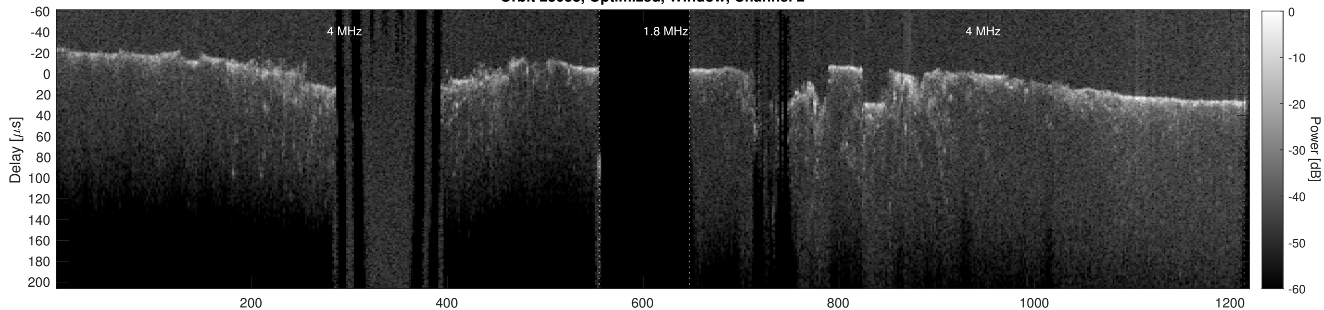
Orbit 23038, Cluttergram
