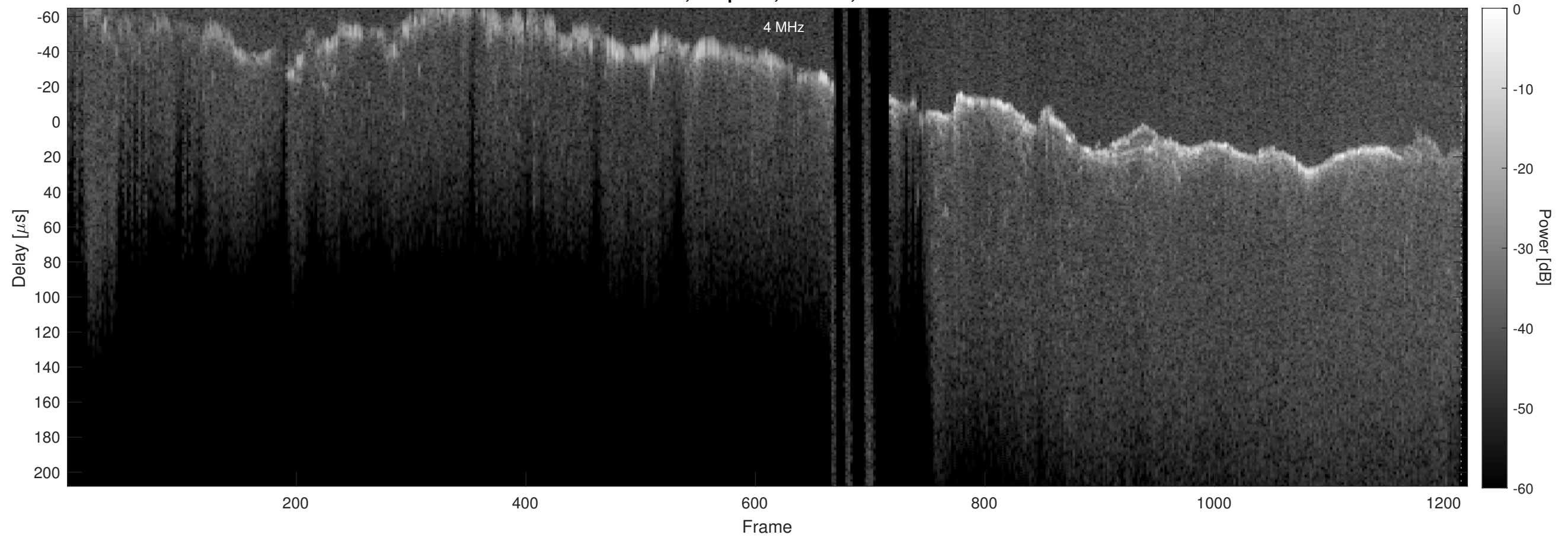
Orbit 23039, Chapman, Window, Channel 2
